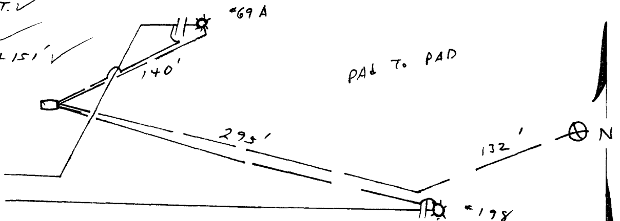
GROUND BED LAYOUT SKETCH
