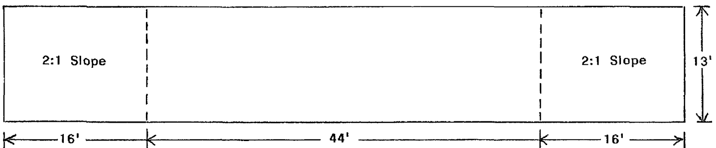
PLAN VIEW
