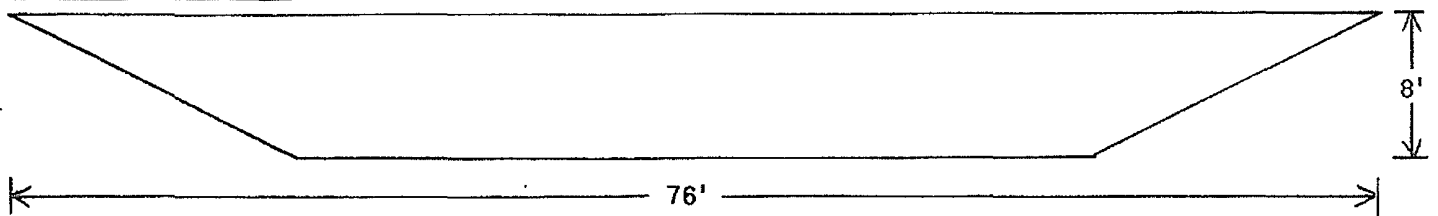
CROSS-SECTION LENGTH
