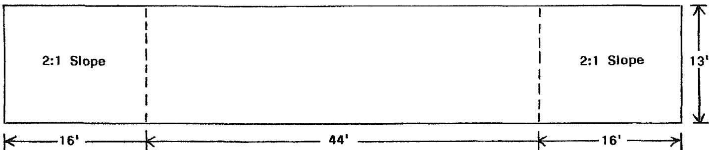
PLAN VIEW
