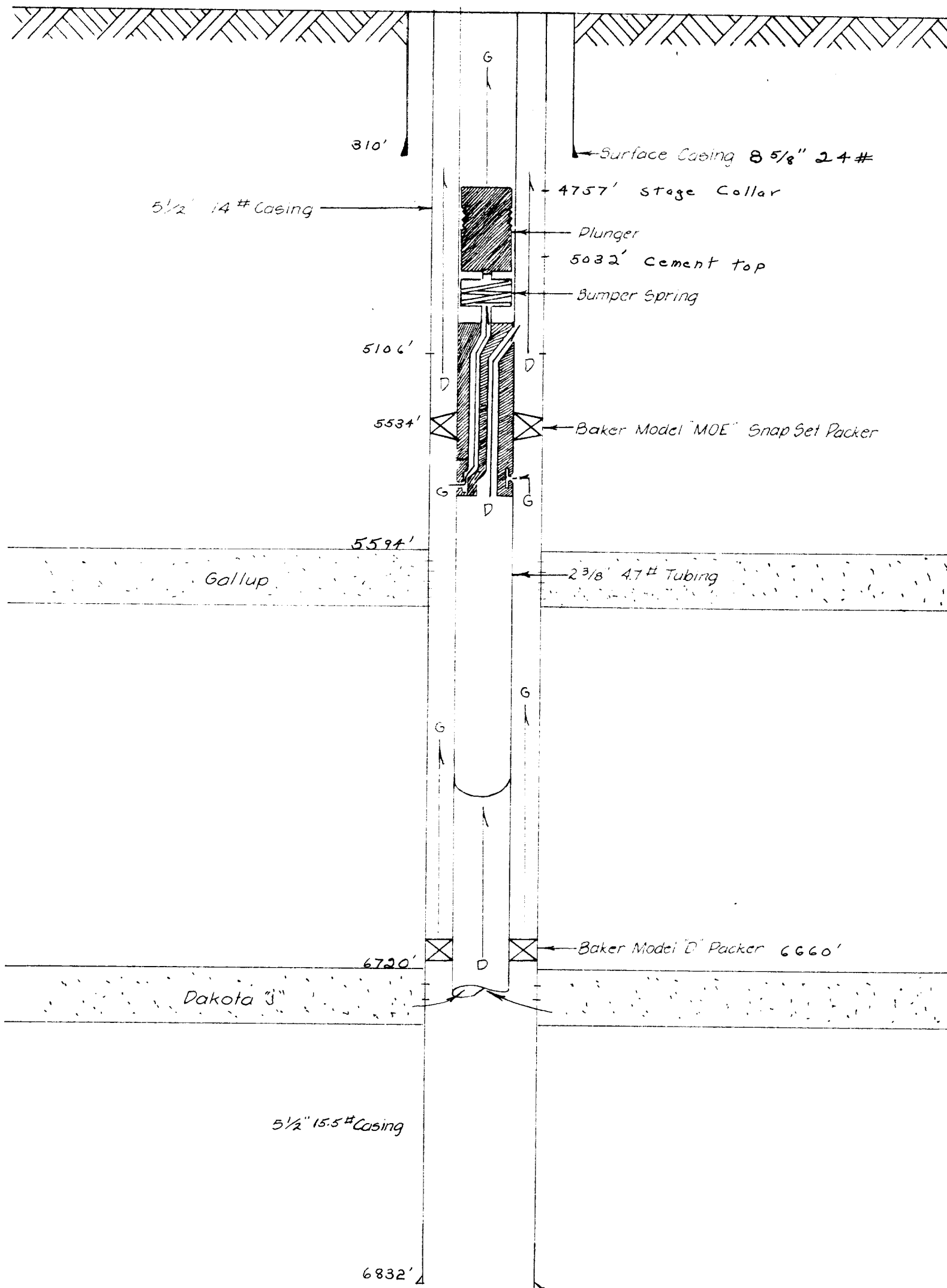
SCHEMATIC DIAGRAM of DUAL COMPLETION of NE. HAYNES No. 6 CONTINENTAL OIL CO. Dakota & Gallup Formations.
