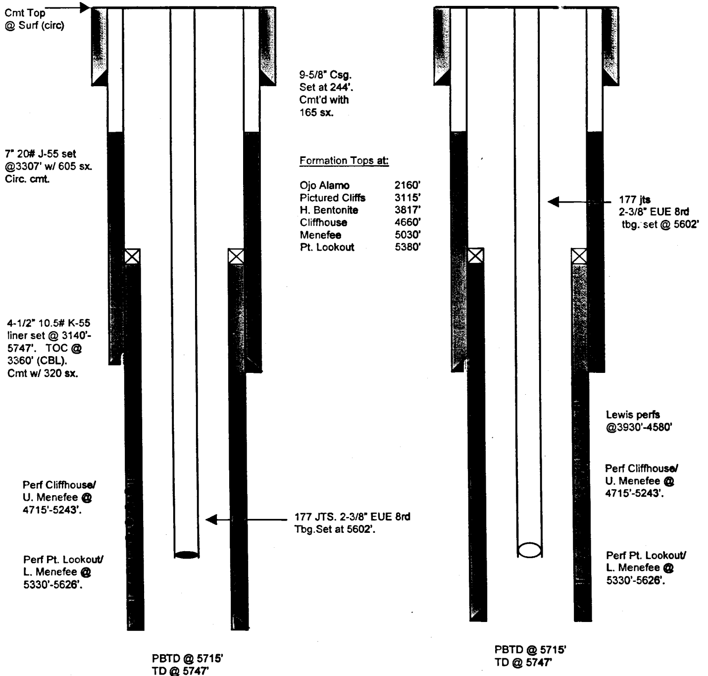
Proposed Schematic
