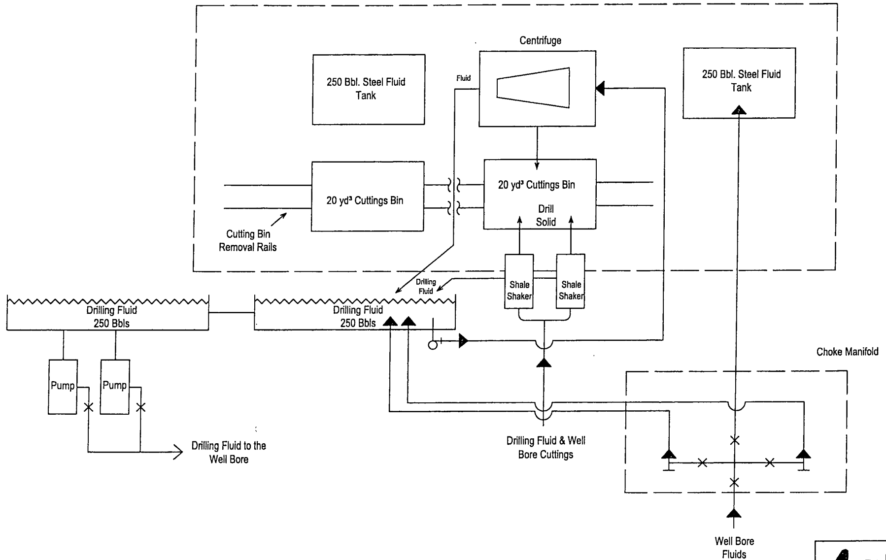
Figure 1 New Mexico Typical Closed-Loop System
