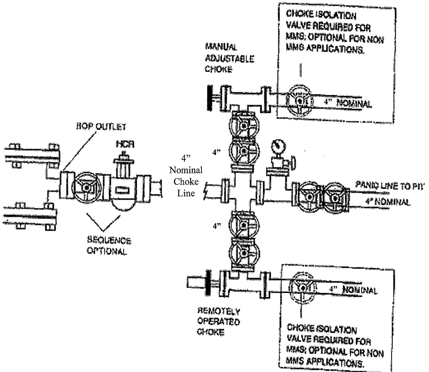
Exhibit E-1 – Choke Manifold Diagram Franklin 18 Federal Com No. 2 Cimarex Energy Co. of Colorado 18-155-31E SHL 1980 FNL & 330 FEL BHL 1980 FNL & 375 FWL Chaves County, NM
