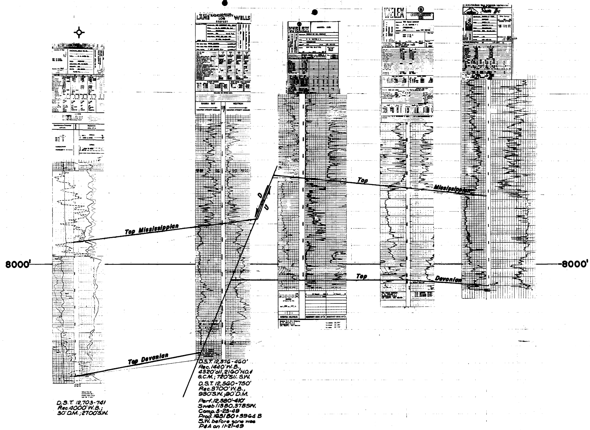
CROSS SECTION A-A' Crossroads Field Area Lea County, New Mexico
