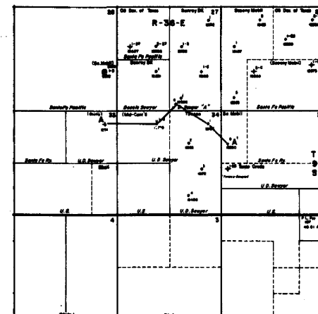
CROSS SECTION A-A' Crossroads Field Area Lea County, New Mexico
