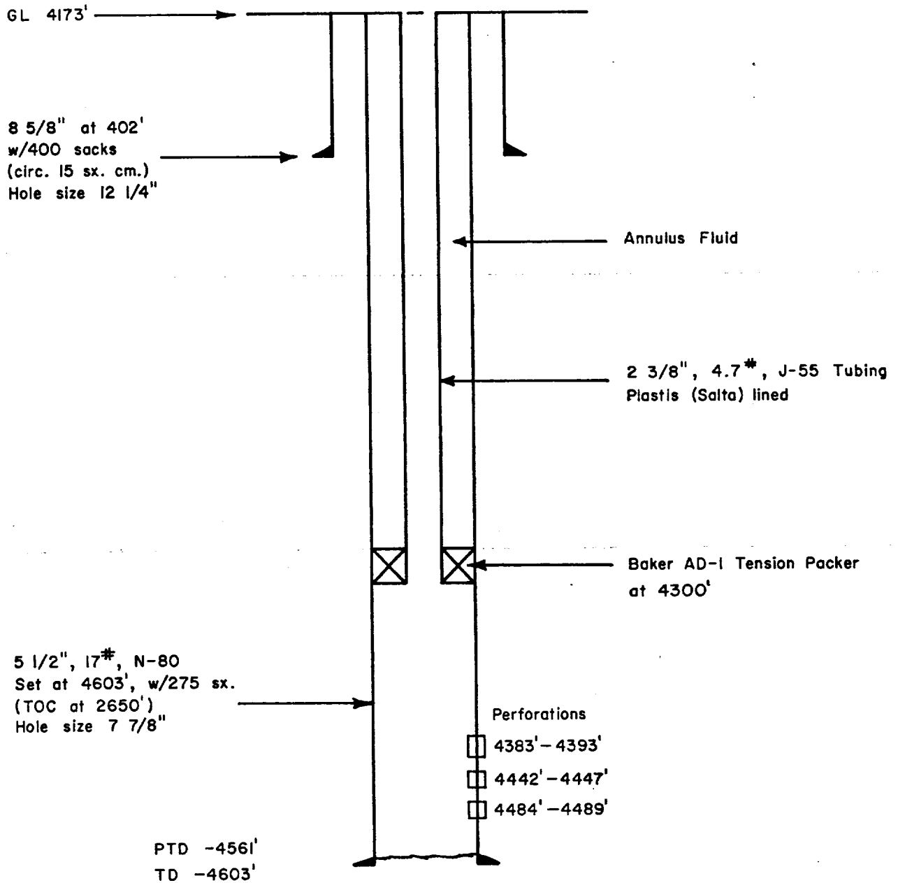
Proposed Completion For Water Injection
