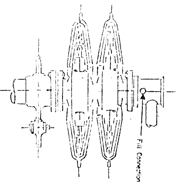
Shaffer Type E Series 900 Hydraulic BOP
