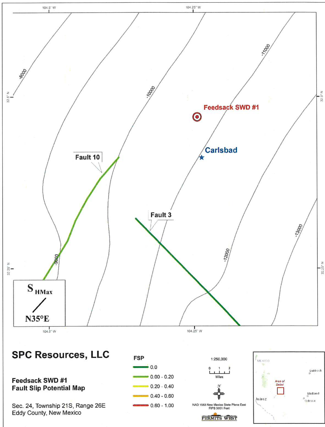
Figure 2. Precambrian fault map of the Feedsack SWD area as mapped by Ewing et al. (1990). Faults are colored based on probability of fault slip as modeled using Fault Slip Potential software (Walsh and Zoback, 2016). Labeled values represent the calculated fault slip potential using the parameters indicated in Table 2. Contours show the top of the Precambrian basement in feet below sea level.
