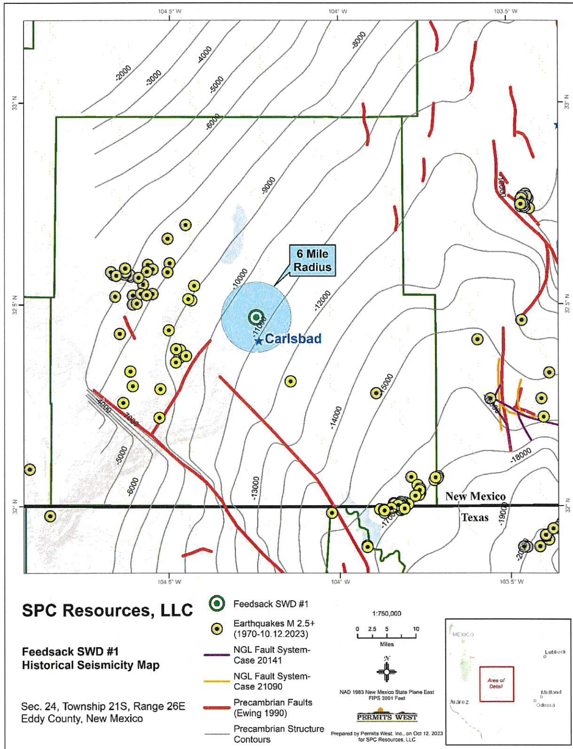
Figure 1. Structural contour map of the Precambrian basement in feet below sea level. Red lines represent the locations of Precambrian basement-penetrating faults (Ewing et al., 1990). Feedsack SWD #1 well lies ~8.9 miles northeast of the closest deeply penetrating fault and ~11.5 miles southeast from the closest historic earthquake.
