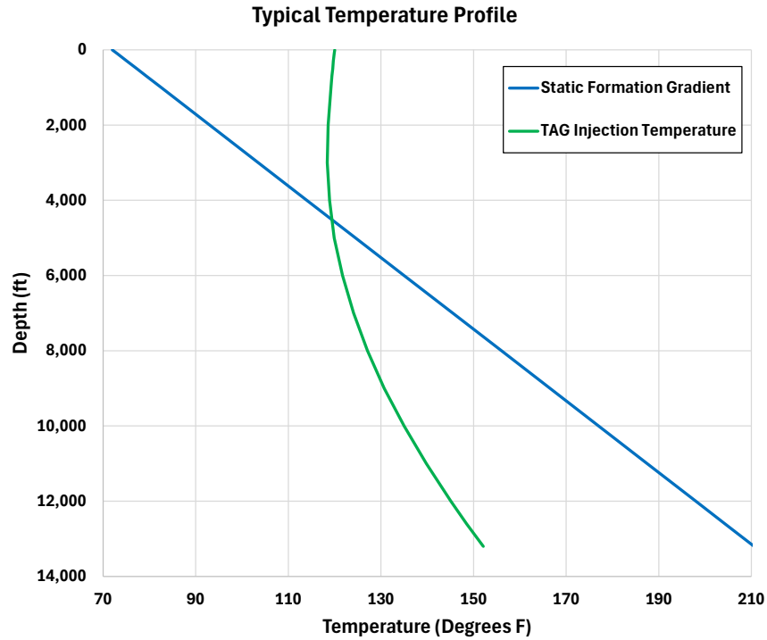
Figure 21 – Temperature Profile
