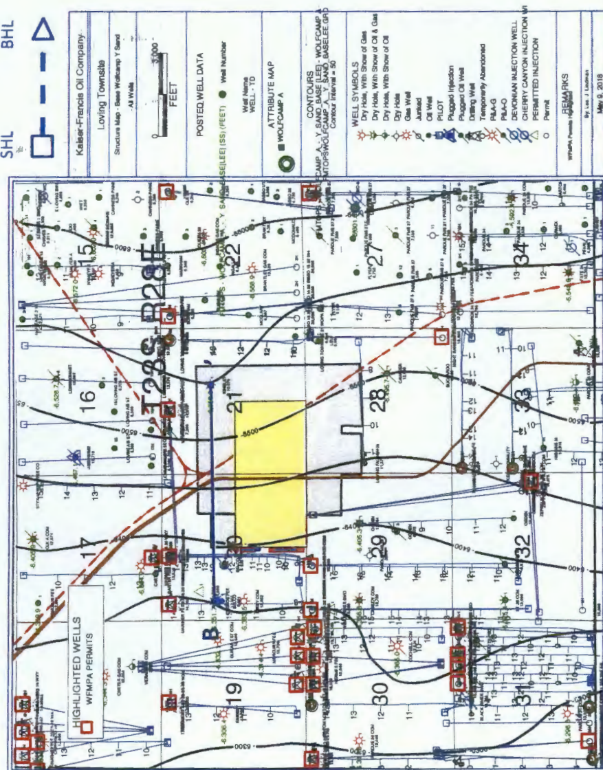
Structure Map (Base Wolfcamp Y Sand - Subsea)
