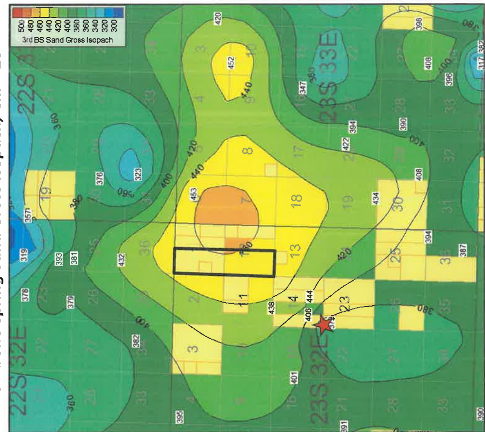
3rd Bone Spring Sand Gross Isopach; C.I. = 20'
