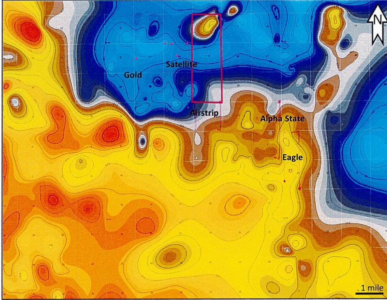
FBSG Sand Isopach
