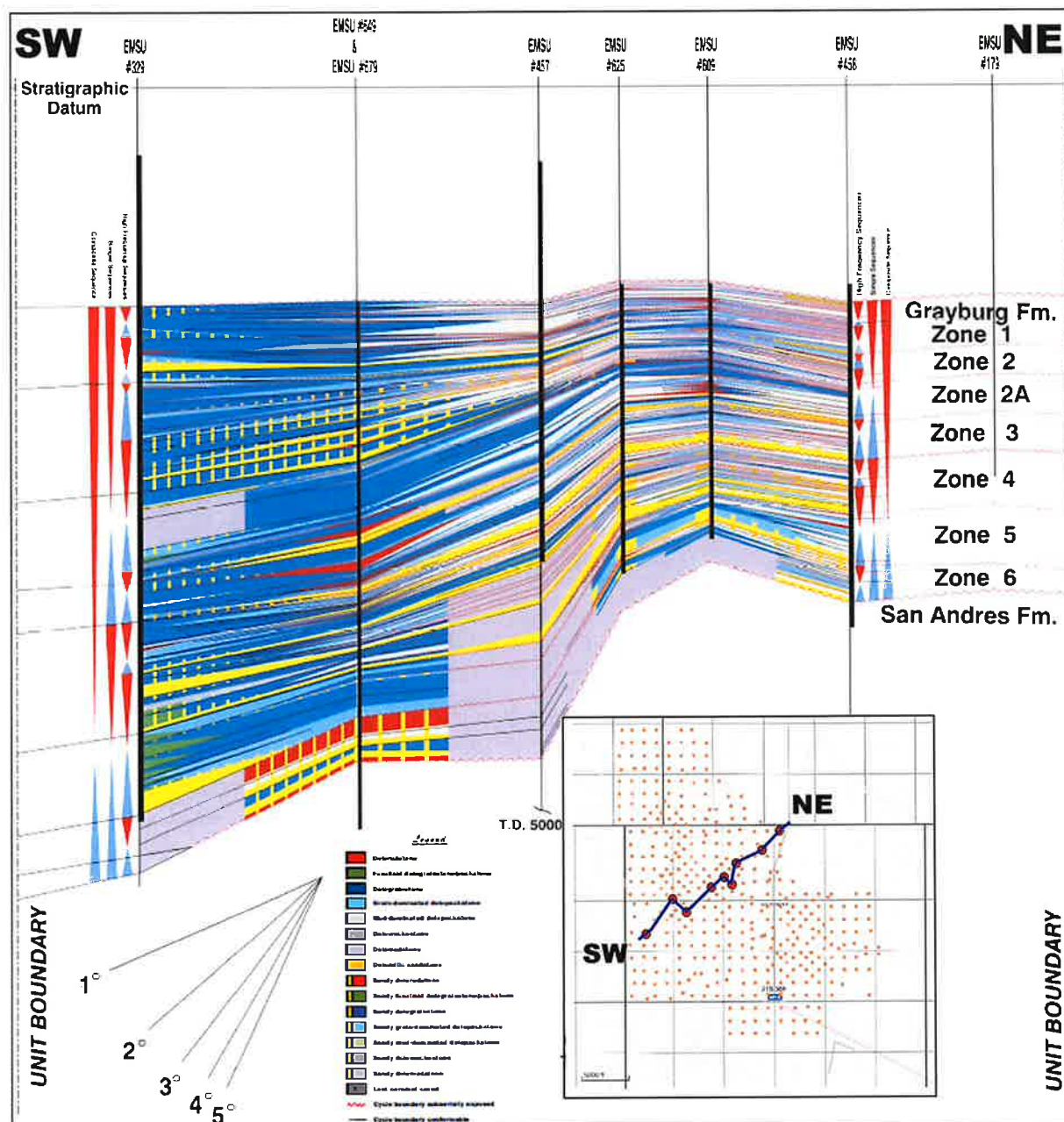
Figure 5.11. Subsurface core descriptions of the Grayburg Formation in dip view through the center of Sive Monument South Unit (EMSU). The Grayburg Formation composite sequence can be divided into a Lower Grayburg stripe sequence and Upper Grayburg stripe sequence. The high frequency sequences are color identified, with five in the Lower Grayburg and five in the Upper Grayburg. These will be reviewed in chapters 6 and 7. Note how the Grayburg Formation stripes and losses accommodation slope (dip) with minimal onlap. The lower two Grayburg Formation high frequency sequences 1-2 (GHFS 1-2) were deposited farther down dip and not in EMSU. The remainder of the Grayburg Formation high frequency sequences 3-5 (GHFS 3-5) flooded onto the northwest corner of the Central Basin Platform.
