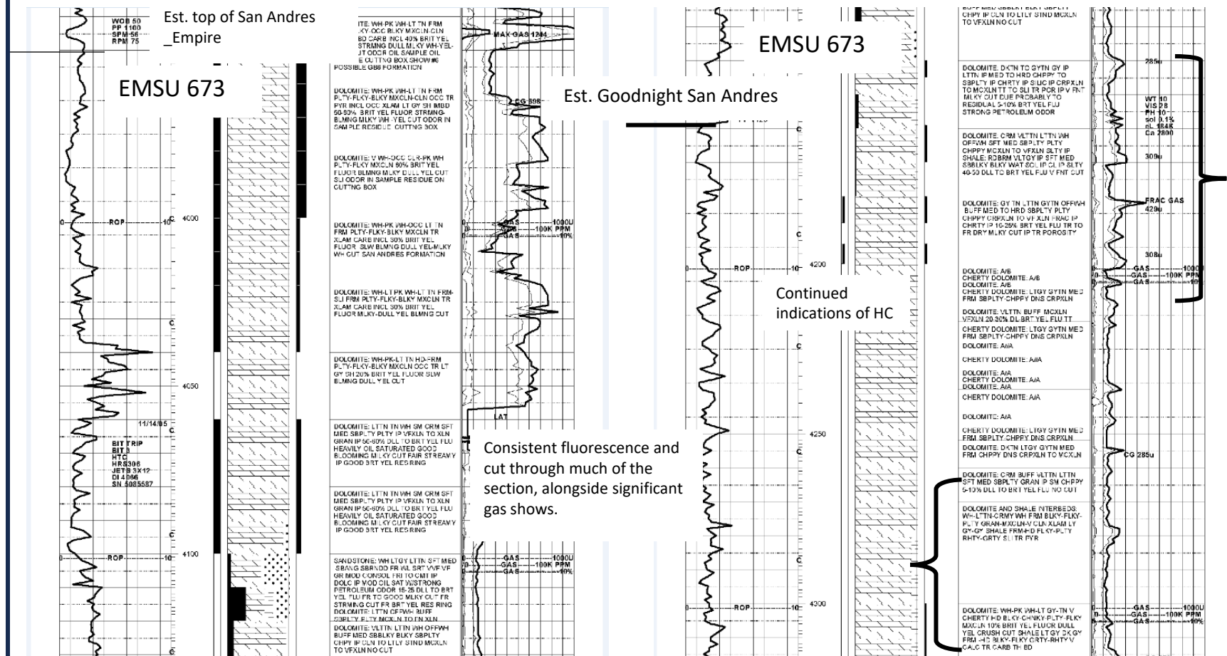
Exhibit L-2: Top of San Andres from Empire and Goodnight interpreters. Reporting of cut fluorescence suggests ROZ or better below each top pick.
