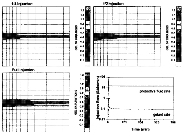
Figure 6. Dual injection of a protective fluid into the upper layer (low permeability) and gelant into the middle layer (high permeability) of a wellbore that has communication behind the pipe.
