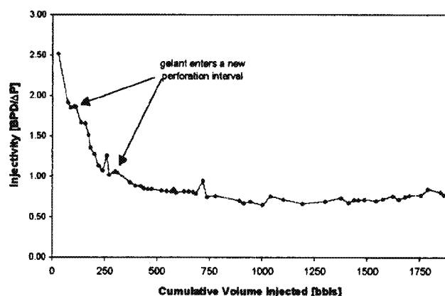
Figure 11. Injectivity decline during gelant injection into EMSU 403.
