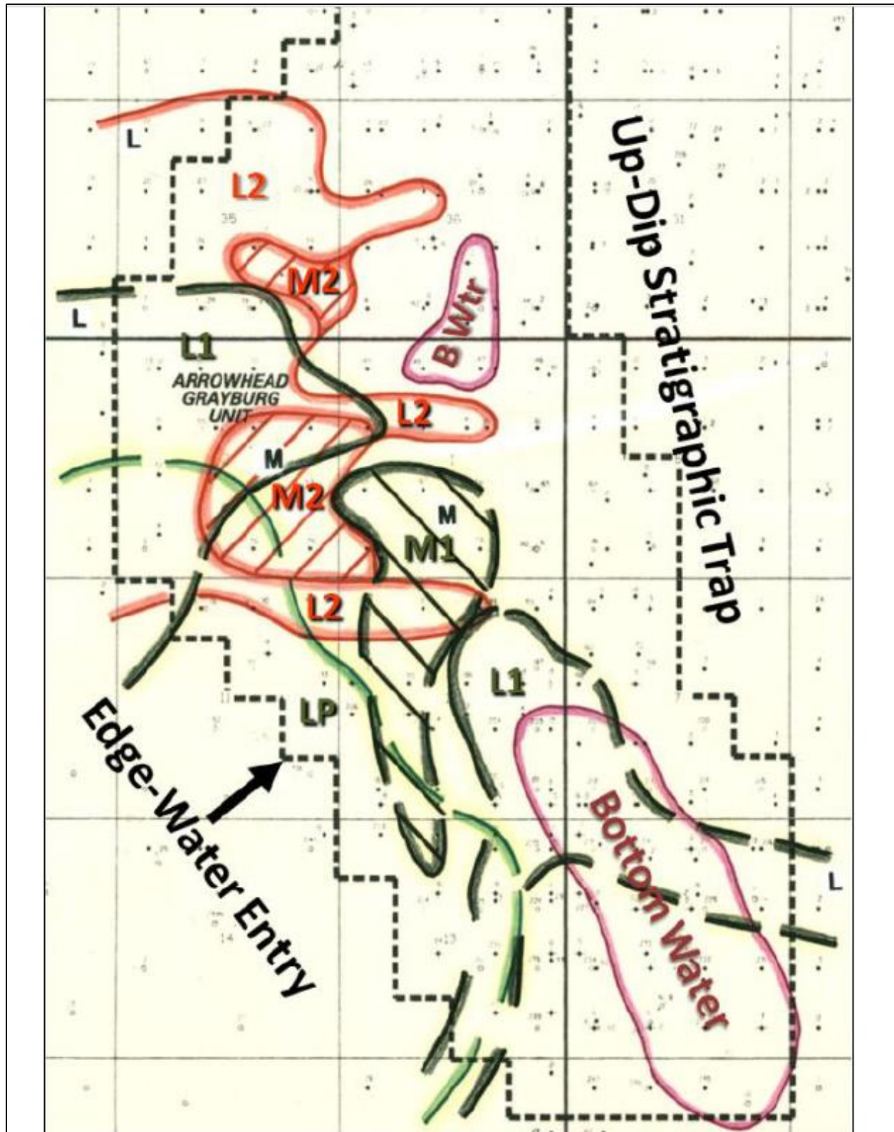
Figure 9.15. Grayburg Formation Arrowhead Grayburg Unit (AGU) with bottom water and four beds of high porosity-permeability dolograins that are each 0.5 m (1.5 ft) thick. These high perm streaks pulled water up-dip into the reservoir by a drop in reservoir pressure during field production. To avoid high water production these beds were not utilized as part of the waterflood.
