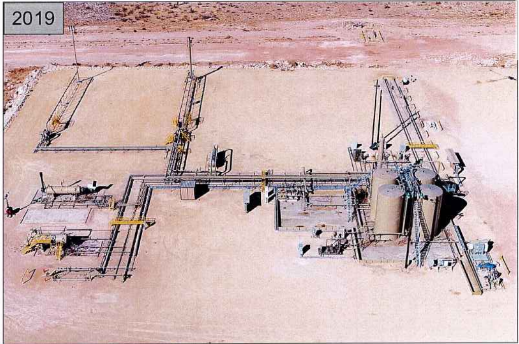
Tanks
