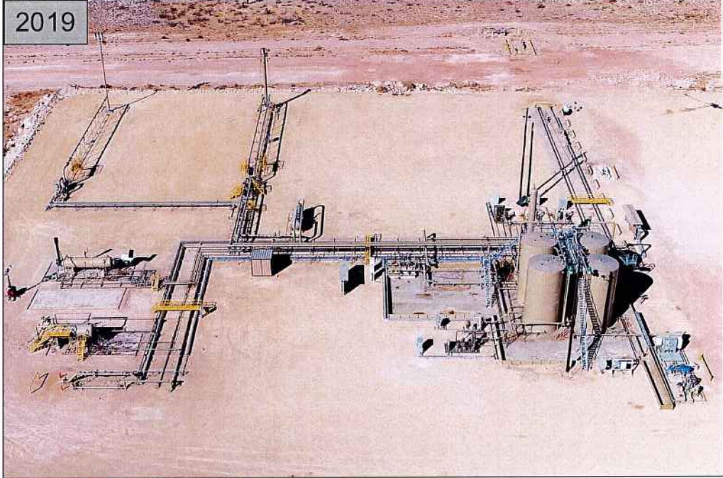
Tanks
