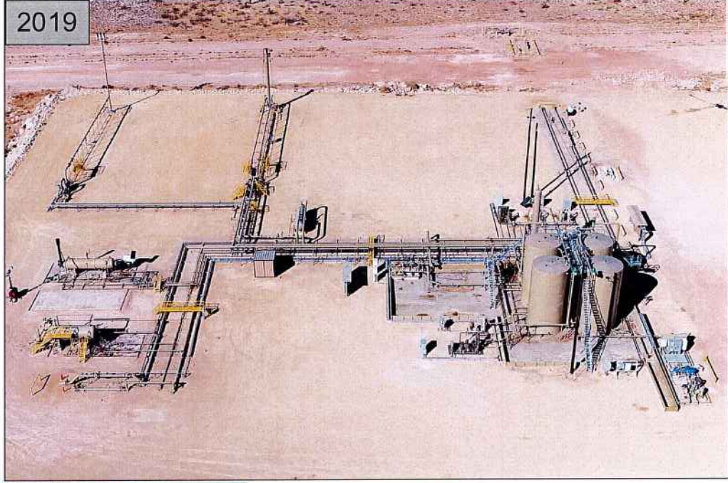
Tanks
