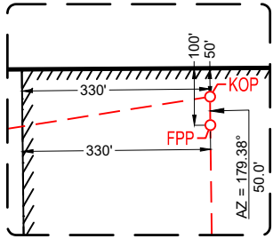
DETAIL VIEW SCALE: 1" = 300'
