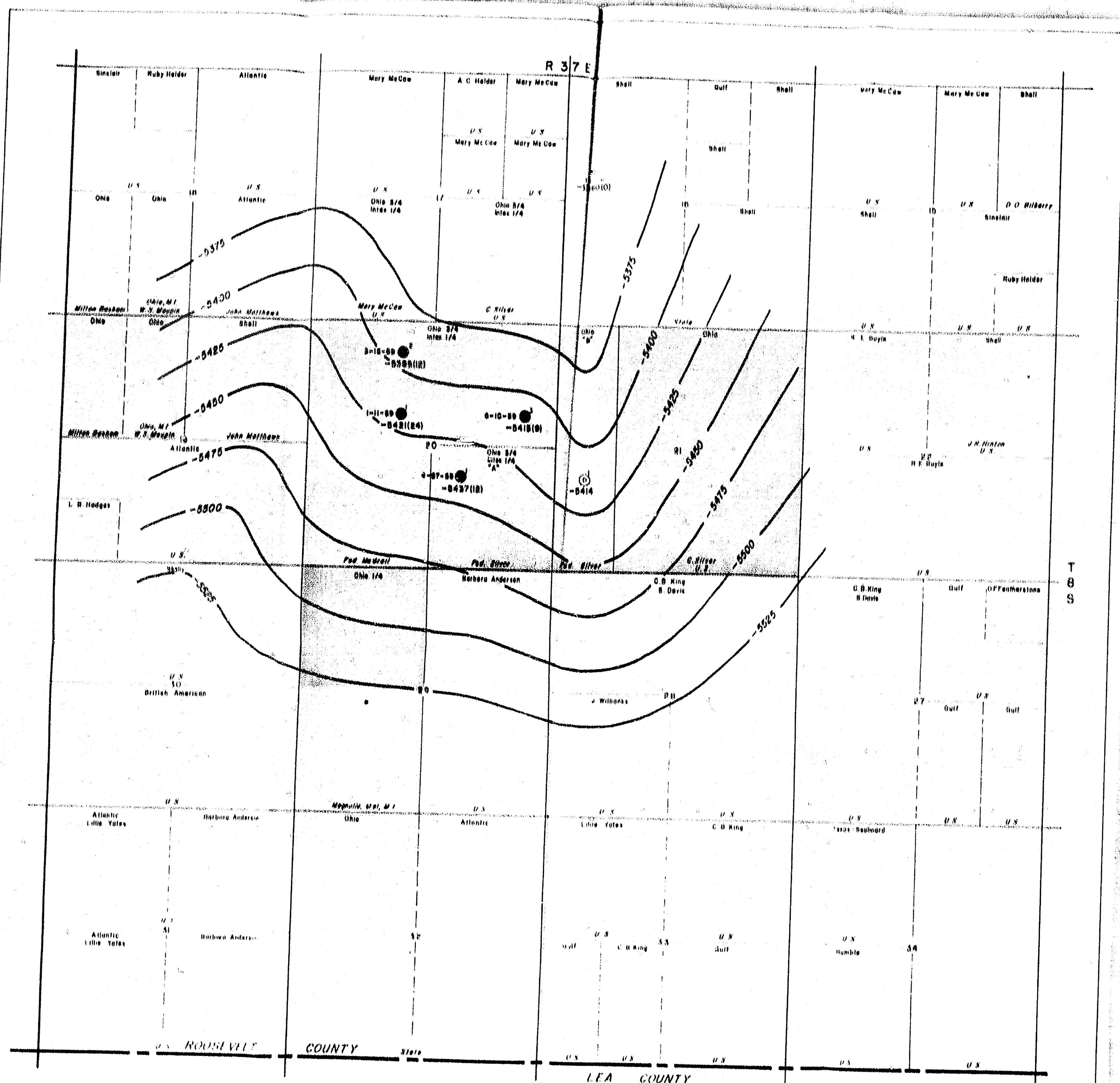
CONTOURED ON TOP OF ROUGH "C" FORMATION CONTOUR INTERVAL --- 25' BLUIT-PENN POOL ROOSEVELT COUNTY, NEW MEXICO SCALE 0 1000 2000 The Price Oil Company - Houston, Texas Computed from County Map MHOCC CASE NO. _____ OHIO EXHIBIT NO. _____ DATE _____
