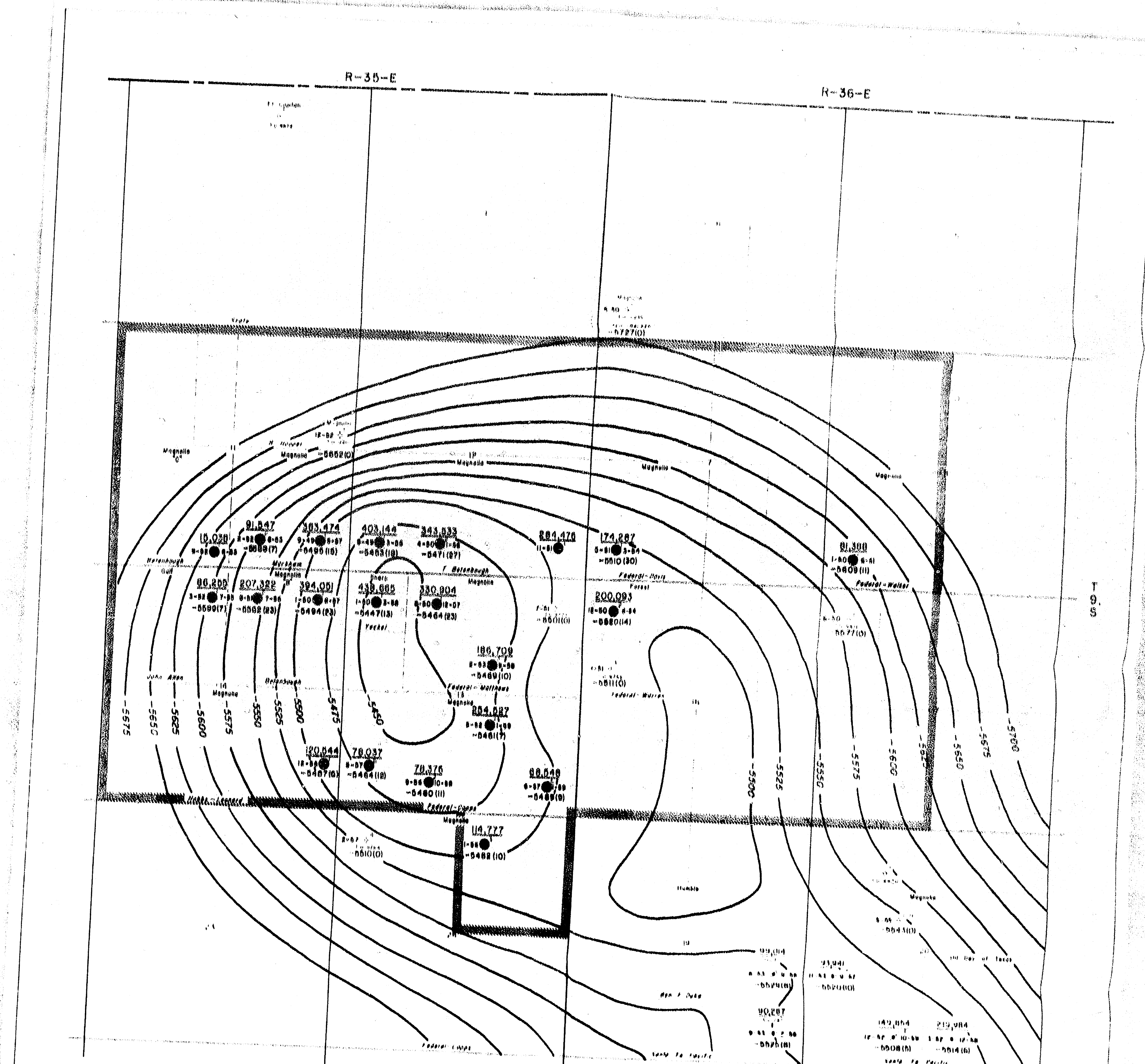
CONTOURED ON TOP OF ROUGH "C" FORMATION CONTOUR INTERVAL --- 25' BOUGH POOL LEA COUNTY, NEW MEXICO MHOCC CASE NO. _____ OHIO EXHIBIT NO. _____ DATE _____
