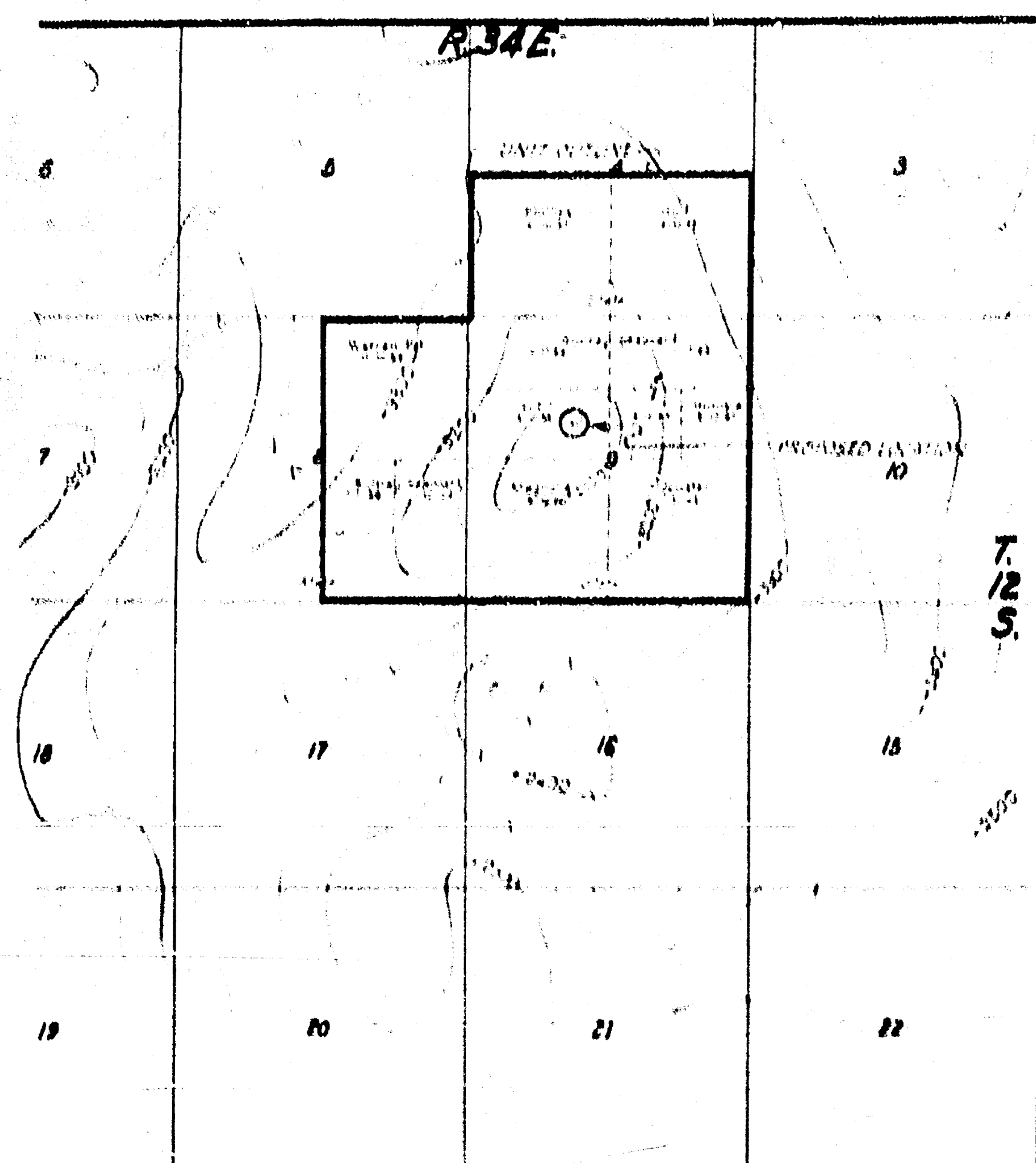
SEISMIC SURVEY EAST BAGLEY AREA LEA COUNTY, NEW MEXICO DEVONIAN CONTOUR INT. 50' SCALE 1:12500
