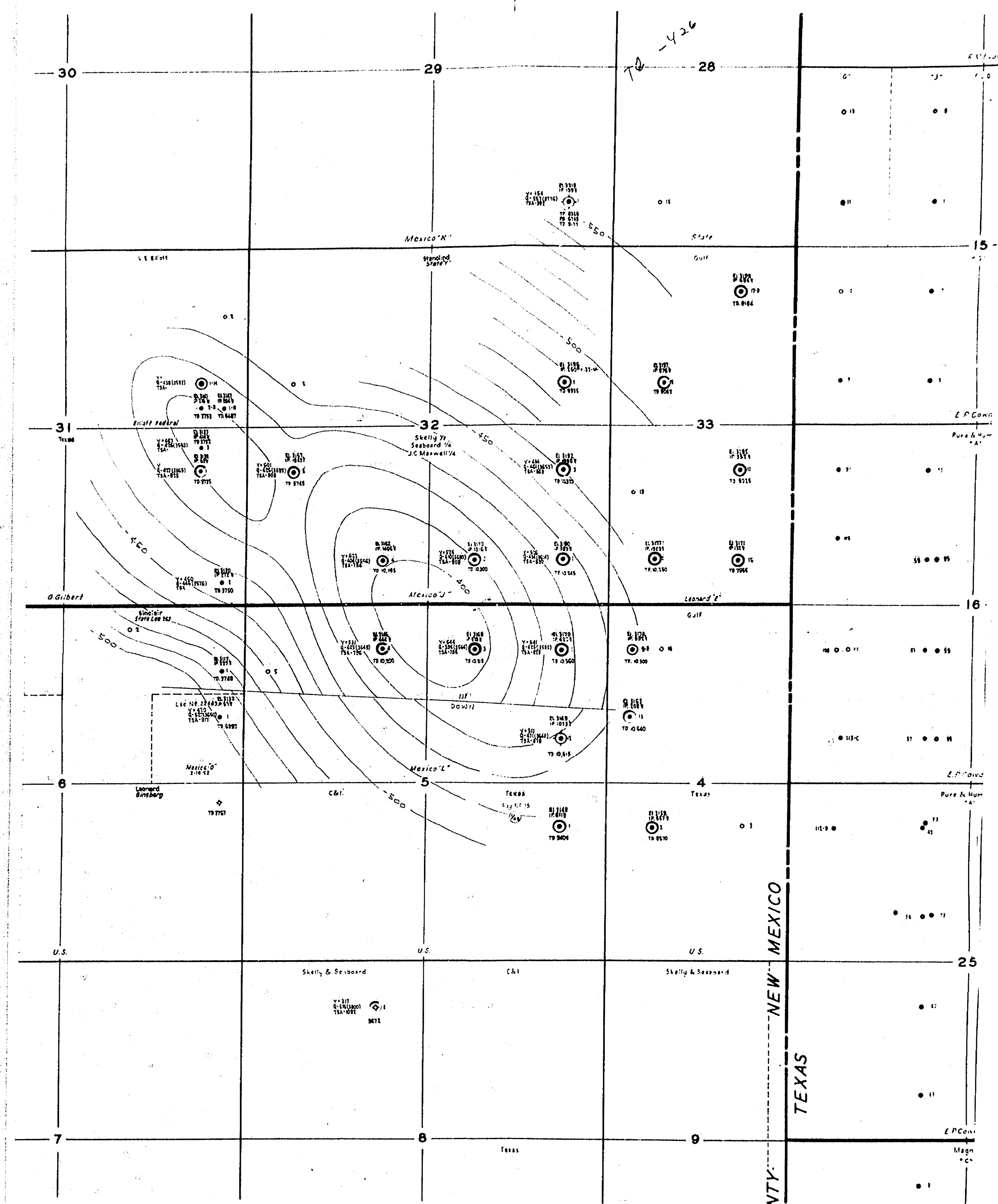
WEST DOLLARHIDE POOL LEA COUNTY, NEW MEXICO Scale 1" = 1000' Contours on Top Quaternary - Contour Interval 100'
