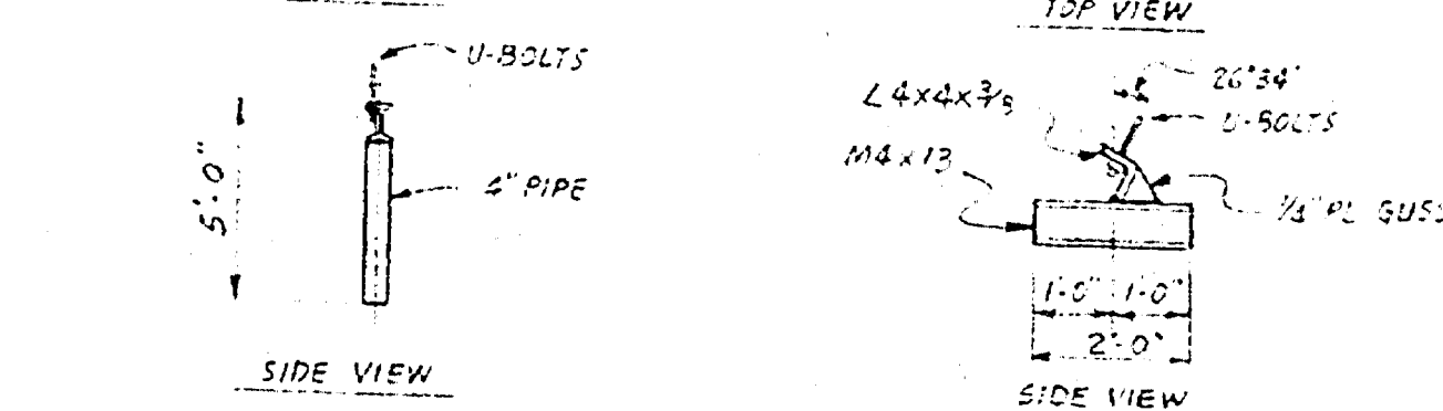
PIPE SUPPORT ON DIKE 1 REQ'D. PER PIT
