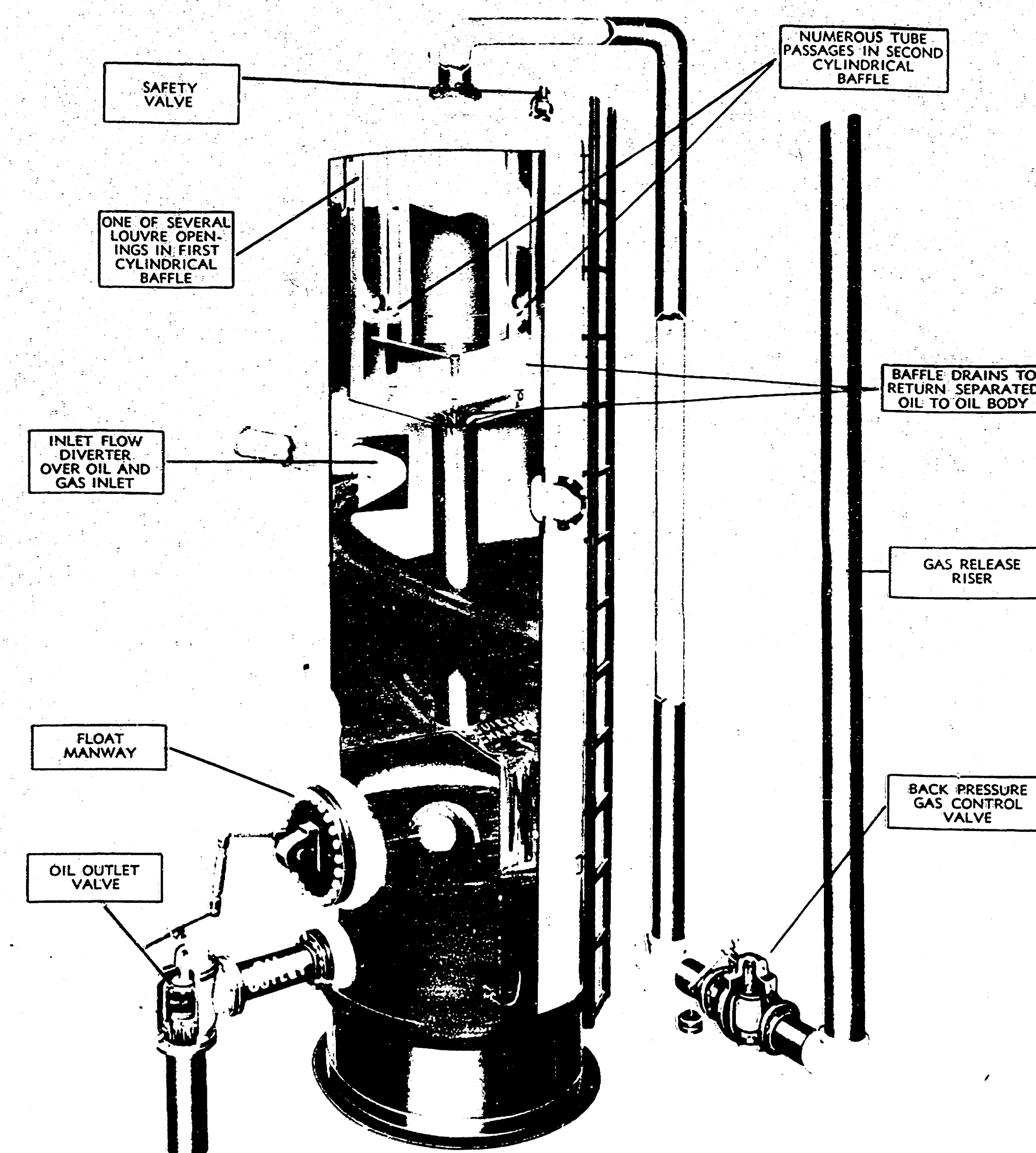
LOW PRESSURE SEPARATOR FLUID FLOW DIAGRAM (Patented)
