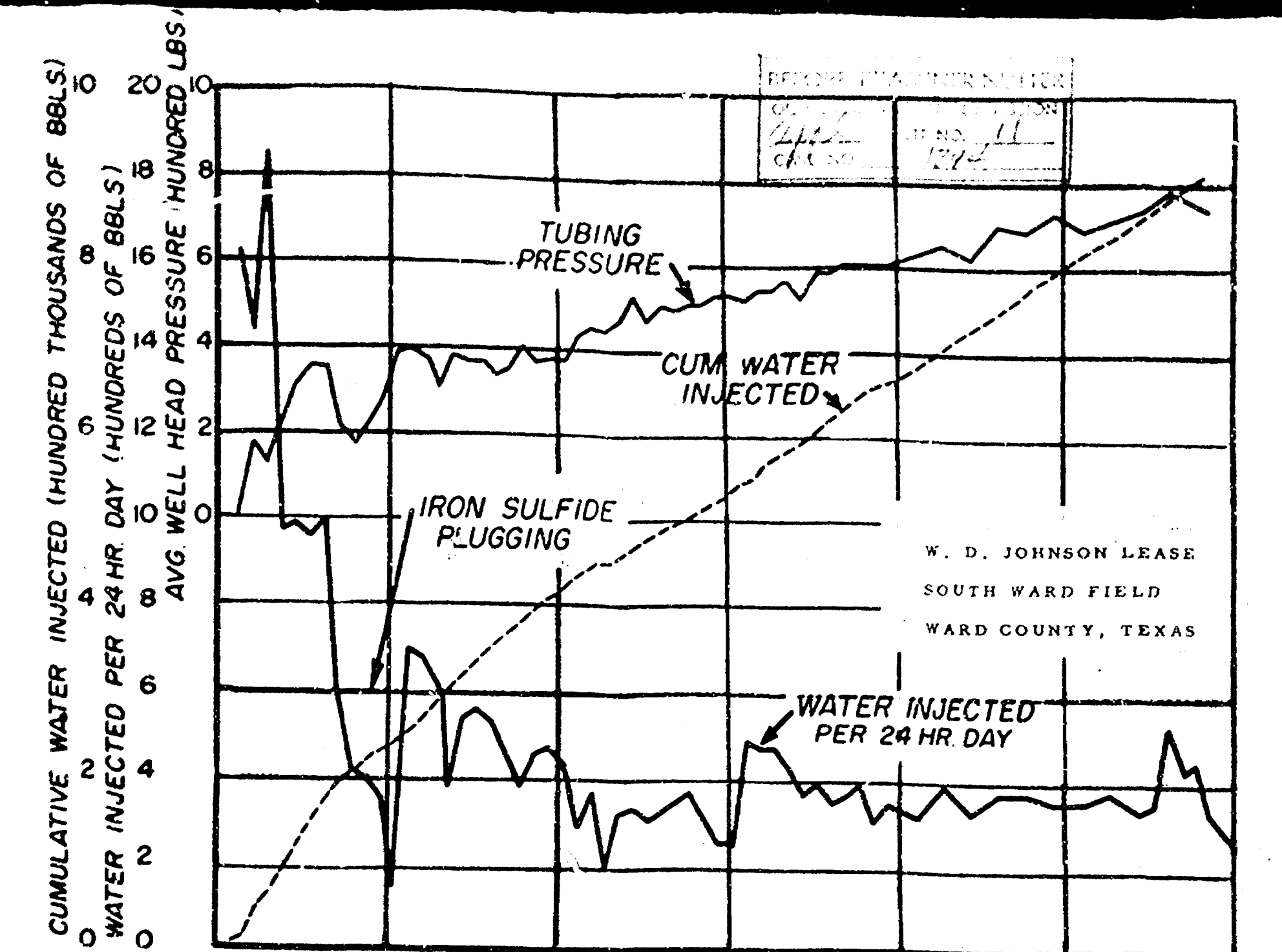
FIG. 3—TYPICAL INJECTION WELL PERFORMANCE DATA. PETROLEUM TECHNOLOGY - October, 1957 - page 283
