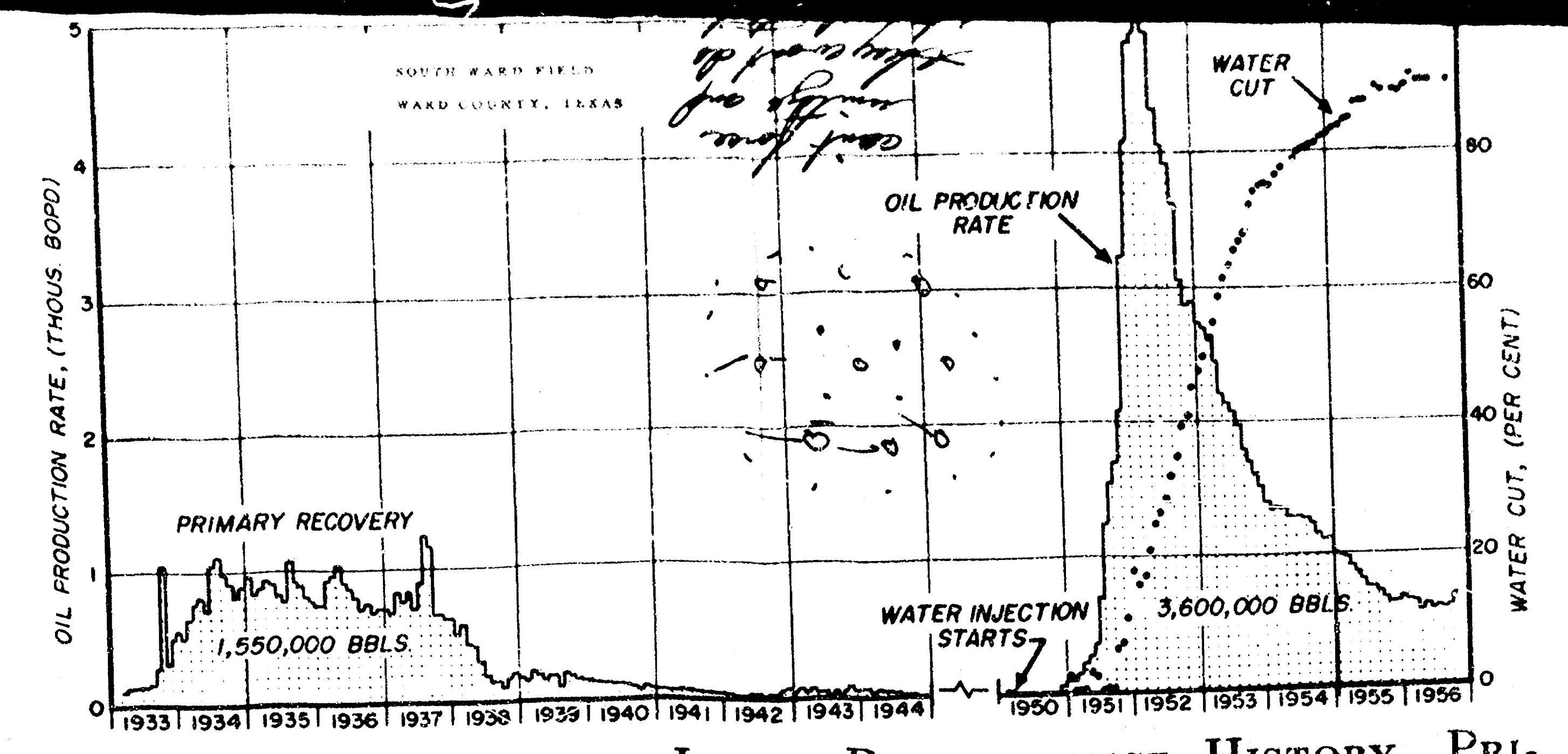
FIG. 4—W. D. JOHNSON LEASE PERFORMANCE HISTORY, PRIMARY AND SECONDARY PRODUCING LIFE.
