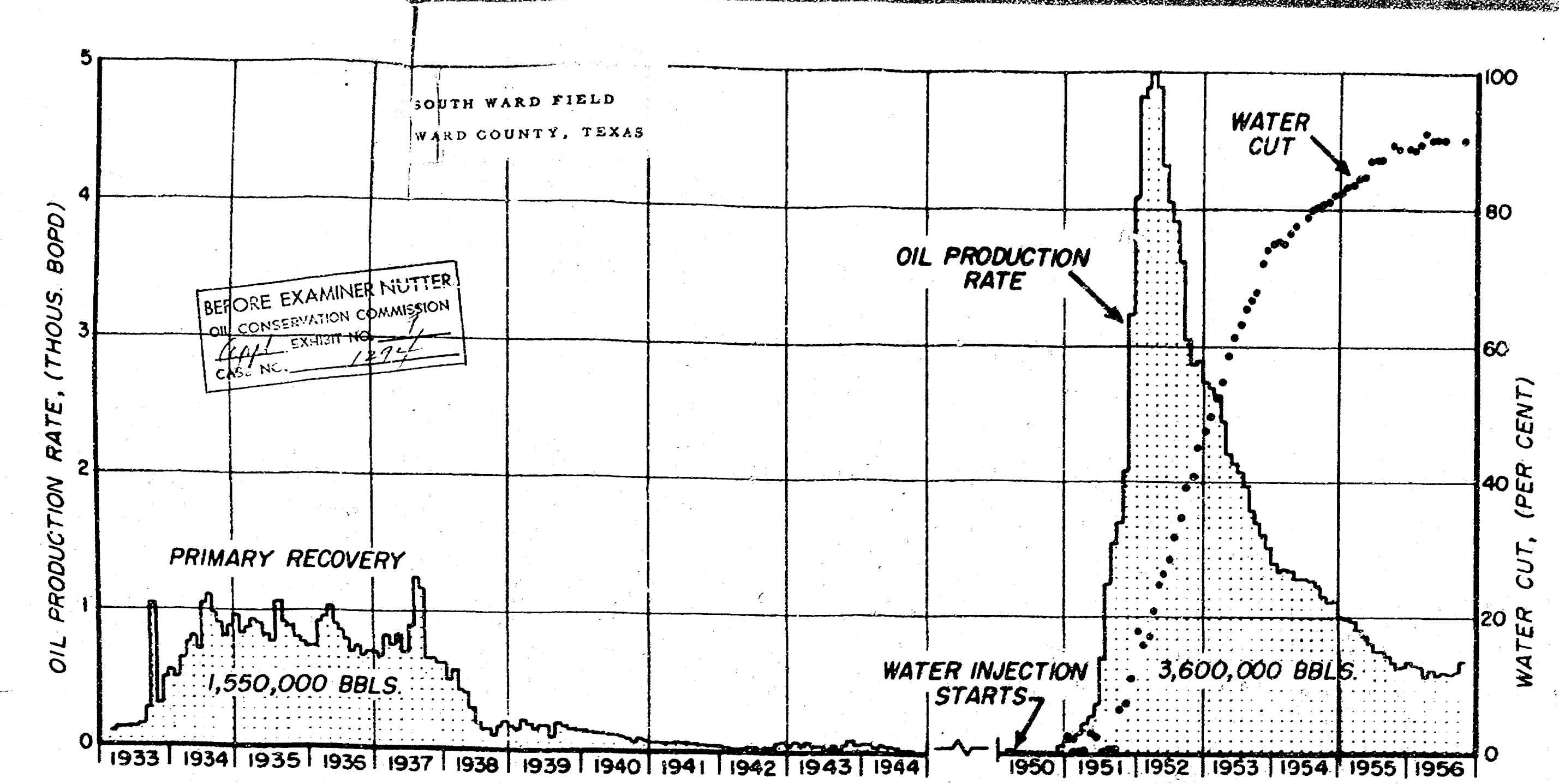
FIG. 4—W. D. JOHNSON LEASE PERFORMANCE HISTORY, PRIMARY AND SECONDARY PRODUCING LIFE.
