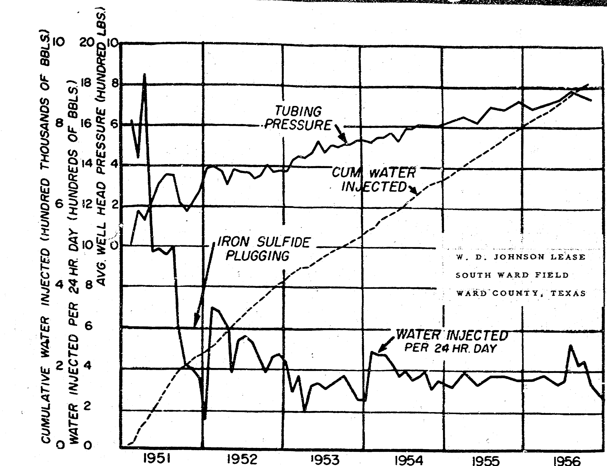
FIG. 3—TYPICAL INJECTION WELL PERFORMANCE DATA. PETROLEUM TECHNOLOGY - October, 1957 - page 283
