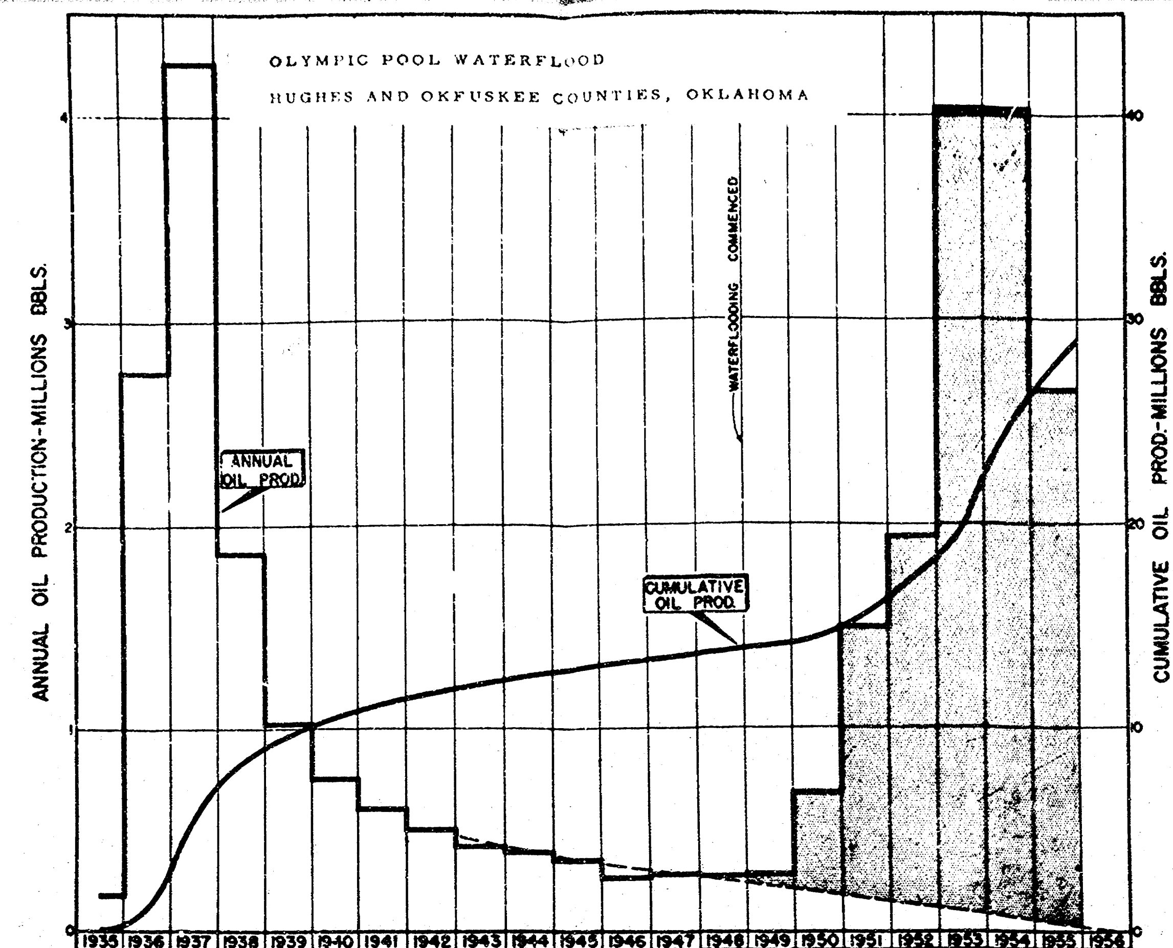
Fig. 4—Primary and secondary production history of entire pool.
