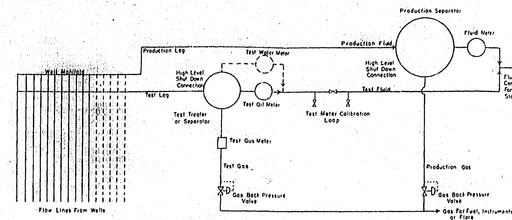
FLOW DIAGRAM OF TYPICAL TESTING STATION ATLANTIC-NAVAJO LEASE HORSESHOE GALLUP FIELD SAN JUAN COUNTY, NEW MEXICO EXHIBIT "B"
