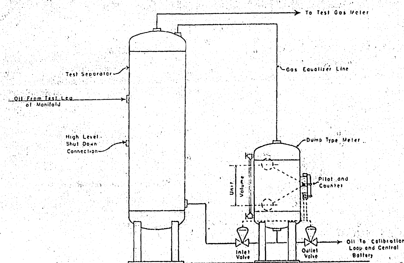
DRAWING OF A DUMP TYPE METER ATLANTIC - NAVAJO LEASE HORSESHOE, GALLUP FIELD SAN JUAN COUNTY, NEW MEXICO EXHIBIT *C*
