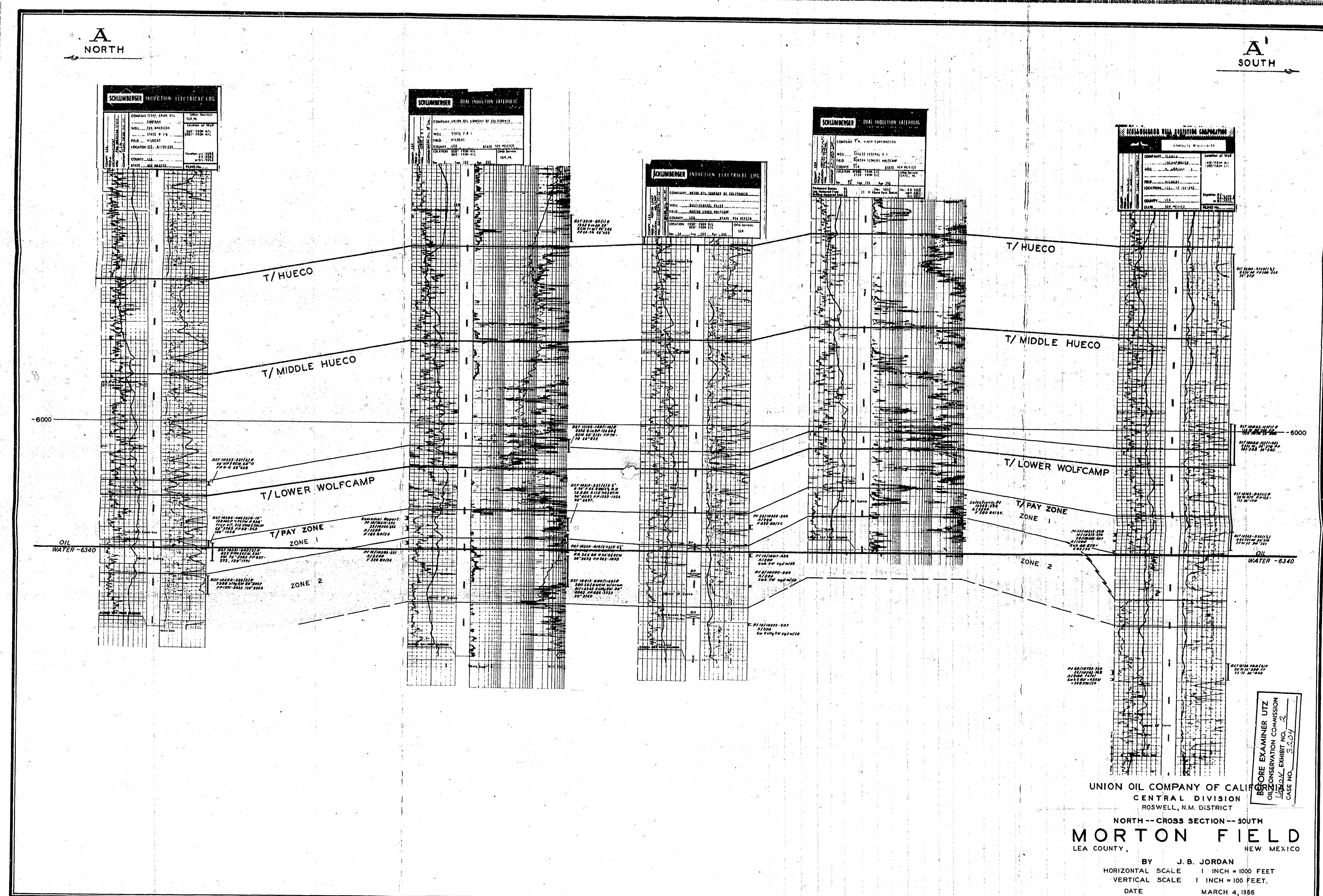
CROSS SECTION A-A'
