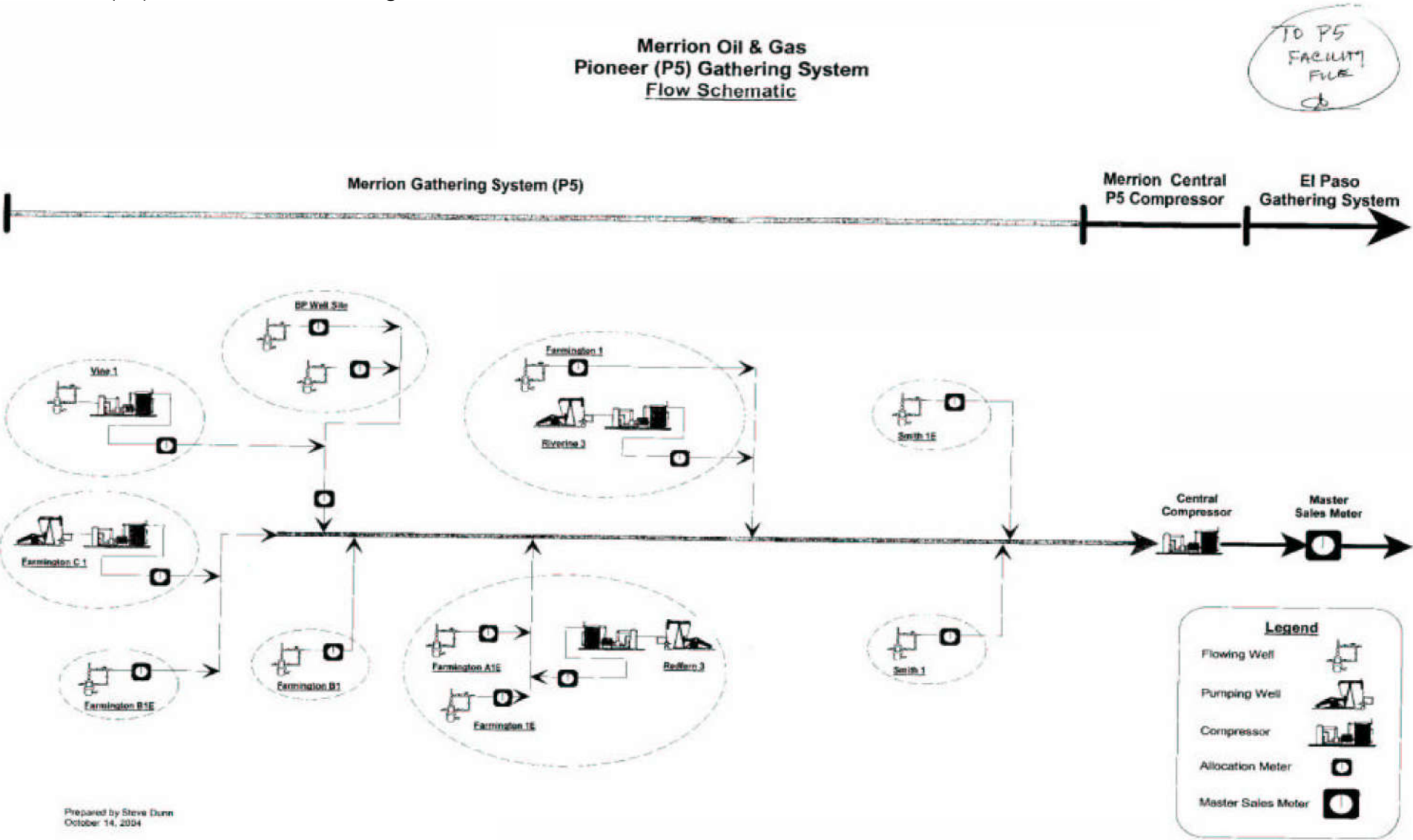
#5 – Delivery System Schematic Diagram
