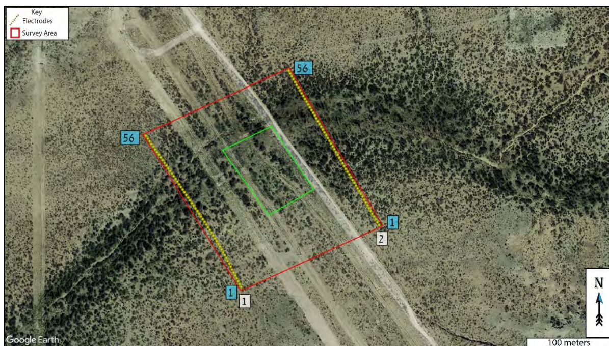
Figure 4: Survey overview. Two survey lines (denoted with white numbers) were conducted with 56 electrodes each at 4-meter spacing (yellow dots denoted with blue numbers). Background image credit: Google Earth. Image date: December 21, 2019. Image datum: WGS-84.
