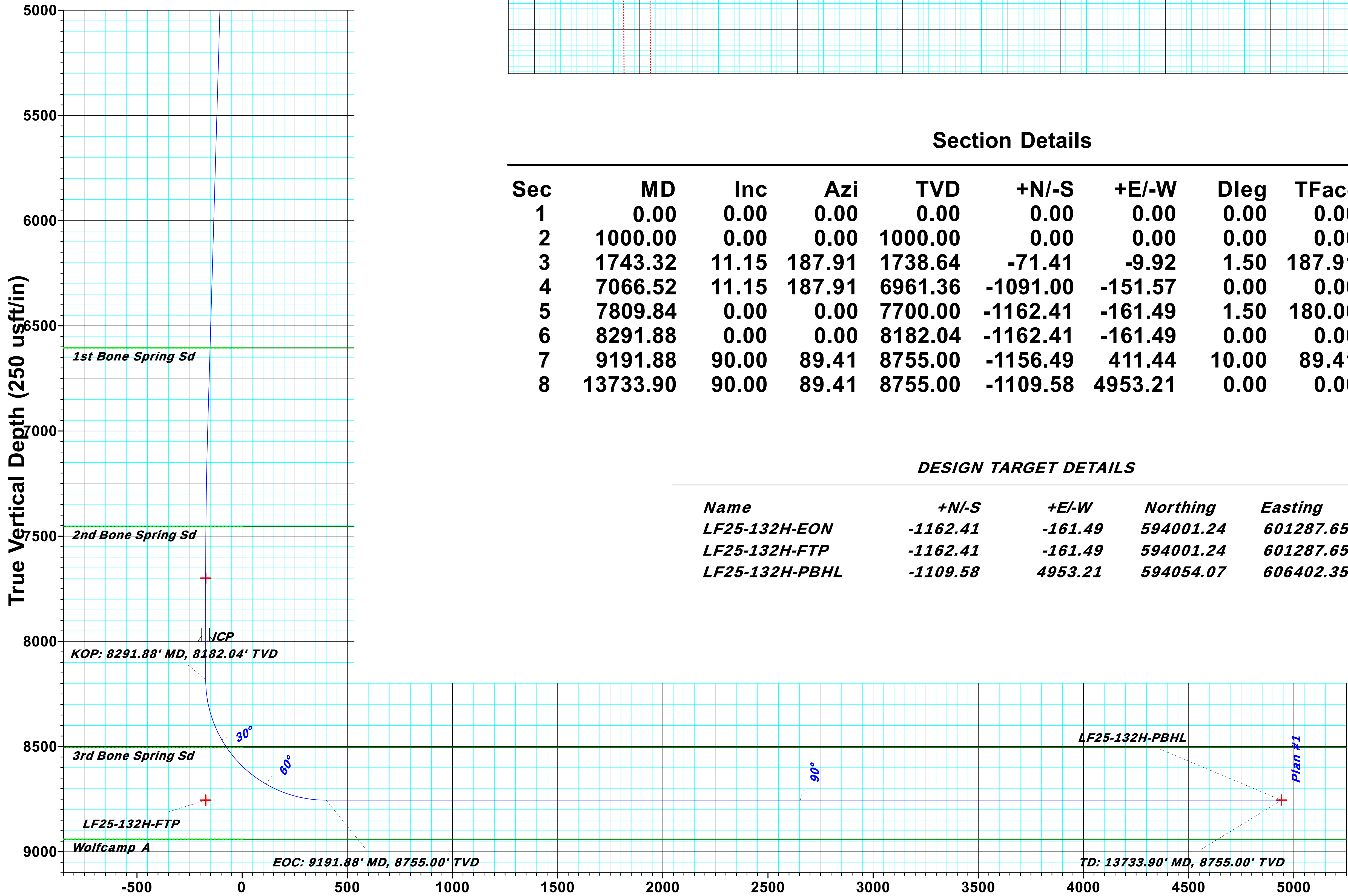
Vertical Section at 89.41° (250 usft/in)
