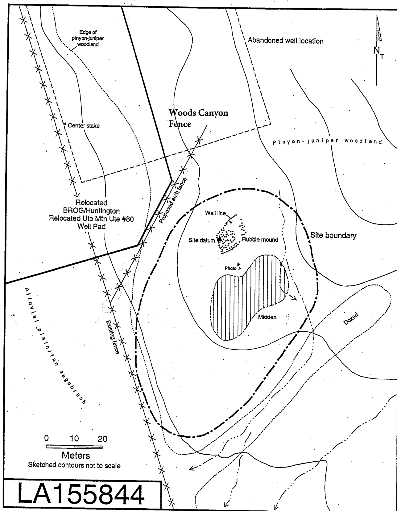
Figure 6. Site plan: LA155844
