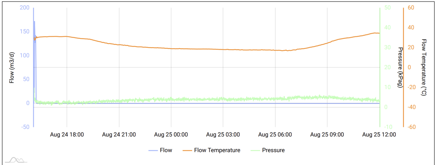
Image 3.1 – Twin Lakes SAU #057 (30-005-61335) Methane Flow/Pressure/Temperature Timeseries
