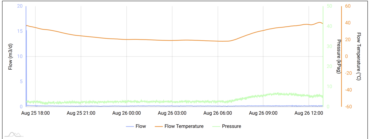
Image 3.1 – Twin Lakes SAU #110 (30-005-61556) Methane Flow/Pressure/Temperature Timeseries
