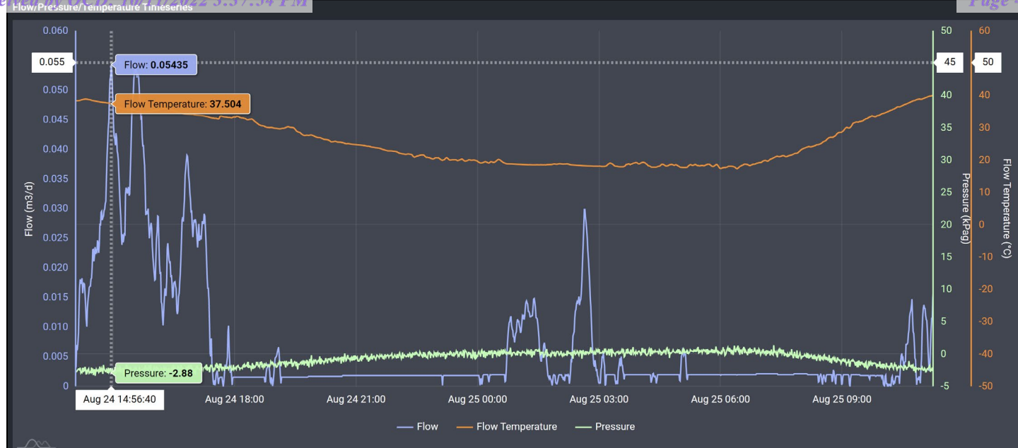
Image 4.1 – Twin Lakes SAU #066 (30-005-60468) Methane Flow/Pressure/Temperature Timeseries
