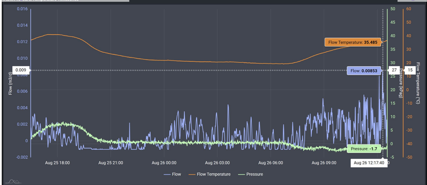
Image 4.1 – Twin Lakes SAU #086 (30-005-60794) Methane Flow/Pressure/Temperature Timeseries &amp; Peak Flow
