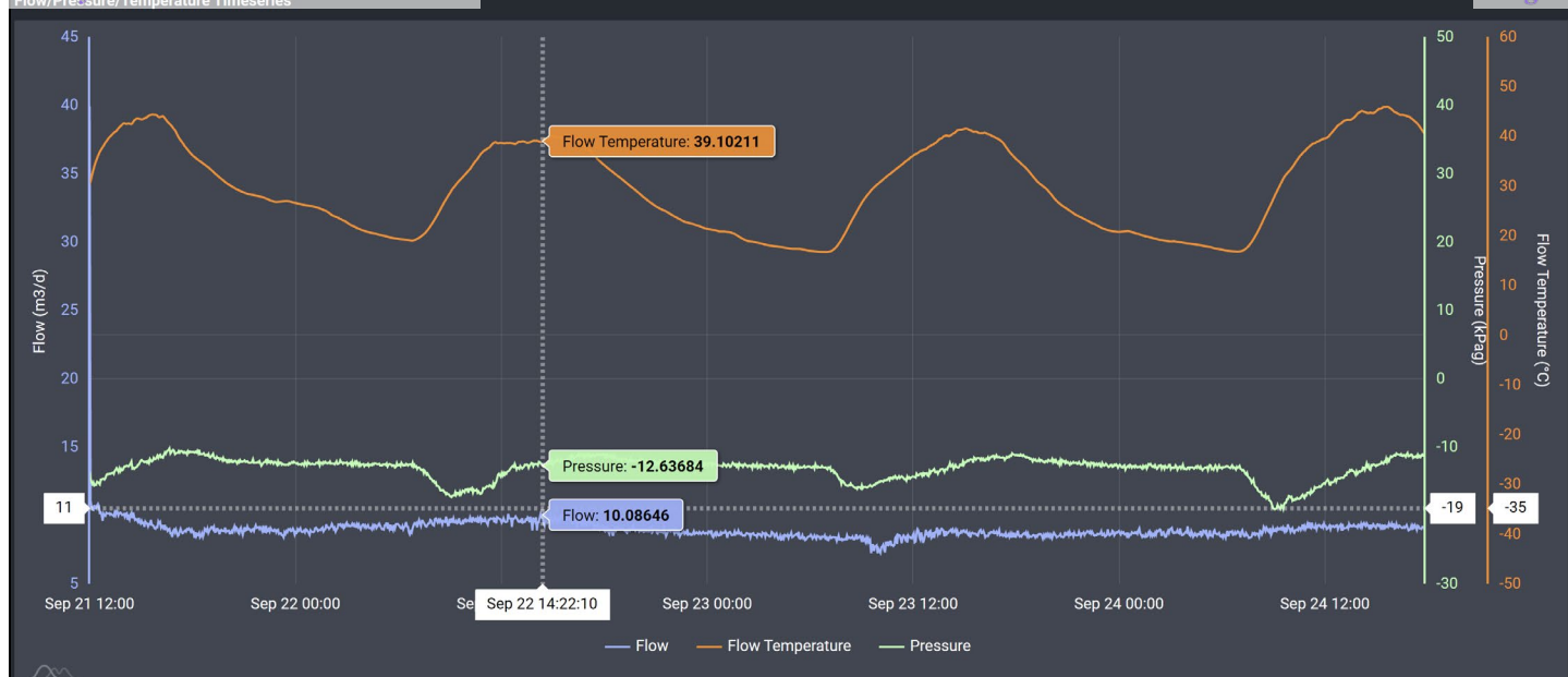
Image 4.1 – State H.L.2 #003 (30-015-25178) Methane Flow/Pressure/Temperature Timeseries &amp; Peak Flow
