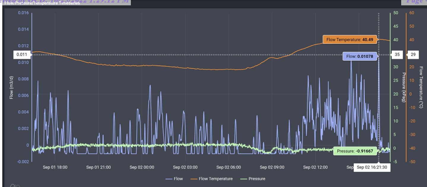
Image 4.1 – Double L Queen #03G (30-005-60079) Methane Flow/Pressure/Temperature Timeseries &amp; Peak Flow
