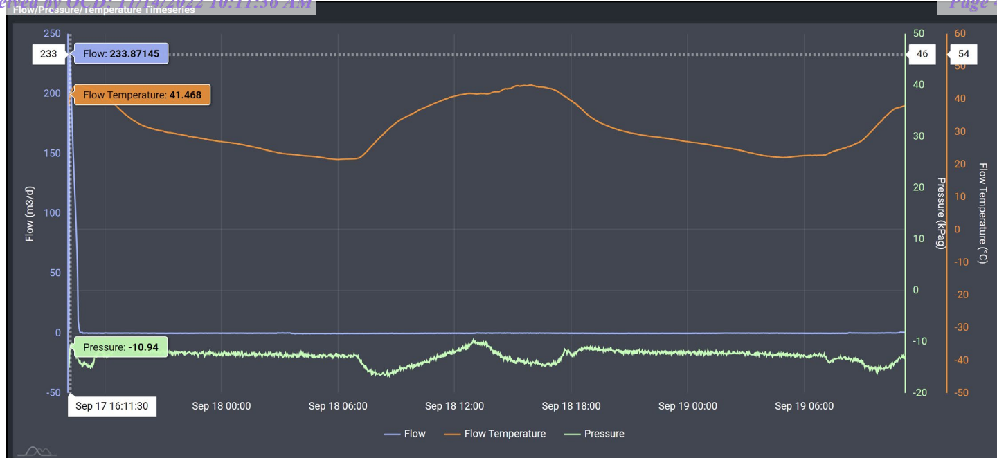
Image 4.1 – Judy #003 (30-025-26262) Methane Flow/Pressure/Temperature Timeseries &amp; Peak Flow
