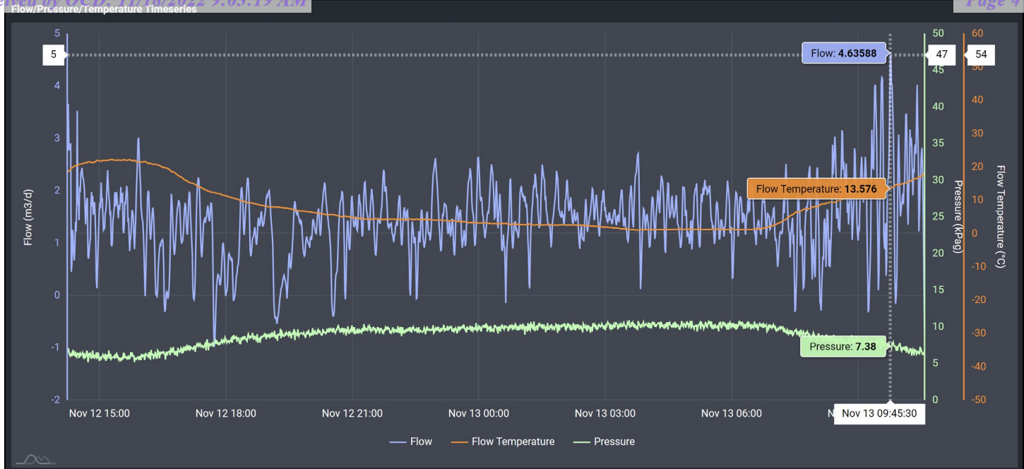
Image 4.1 – Fowler Hair #003 (30-025-11105) Methane Flow/Pressure/Temperature Timeseries &amp; Peak Flow
