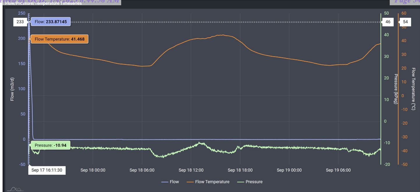
Image 4.1 – Judy #002 (30-025-26262) Methane Flow/Pressure/Temperature Timeseries &amp; Peak Flow
