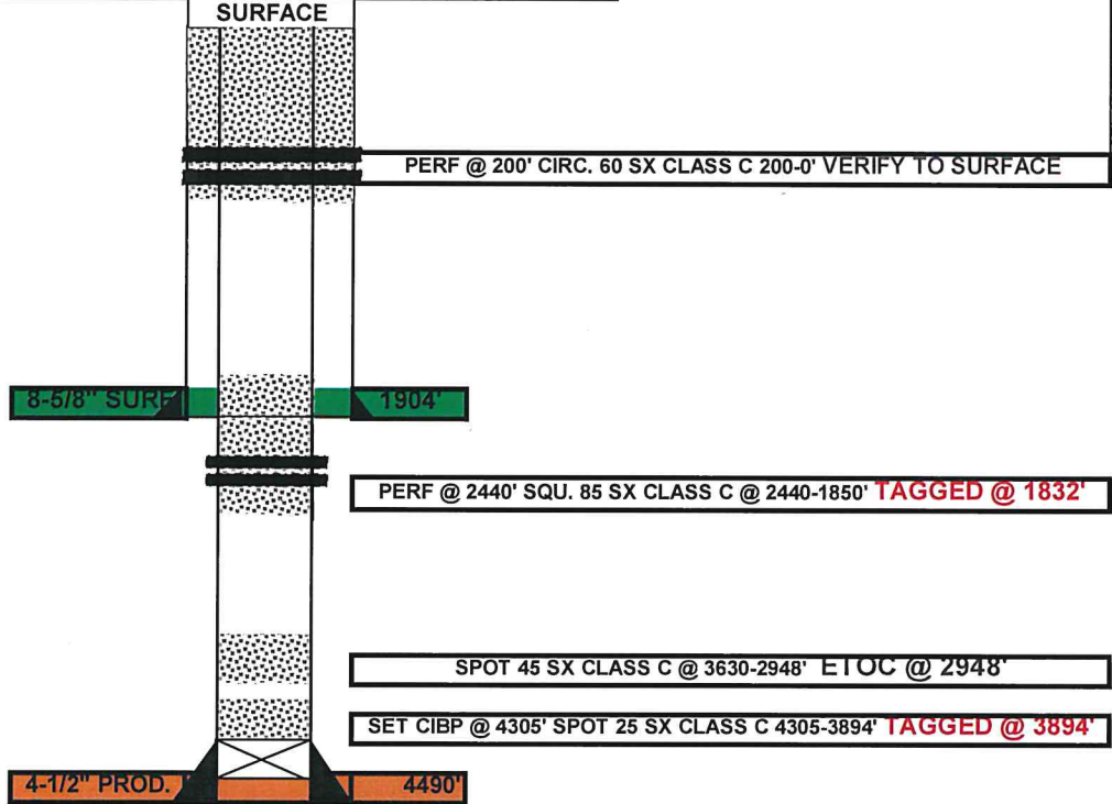
FINAL WELLBORE DIAGRAM
