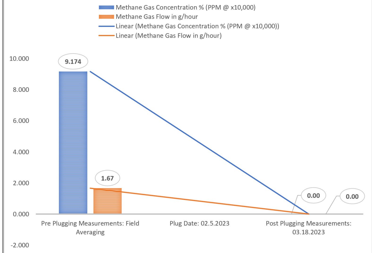
Image 3.1 – O'Brien Fee 18 #003 (30-005-60725) Methane Gas Emissions Reduction Pre Plugging to Post Plugging
