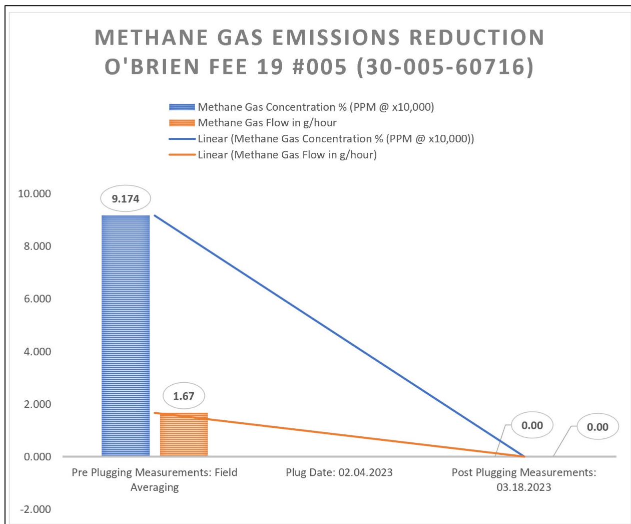
Image 3.1 – O'Brien Fee 19 #005 (30-005-60716) Methane Gas Emissions Reduction Pre Plugging to Post Plugging
