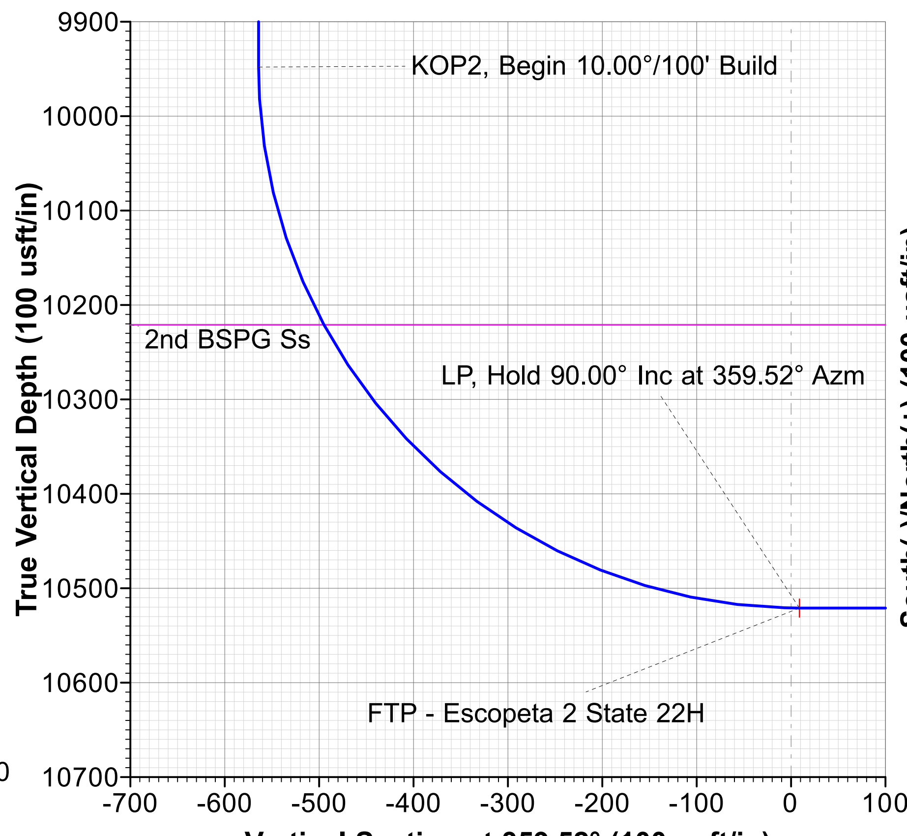
Vertical Section at 359.52° (100 usft/in)
