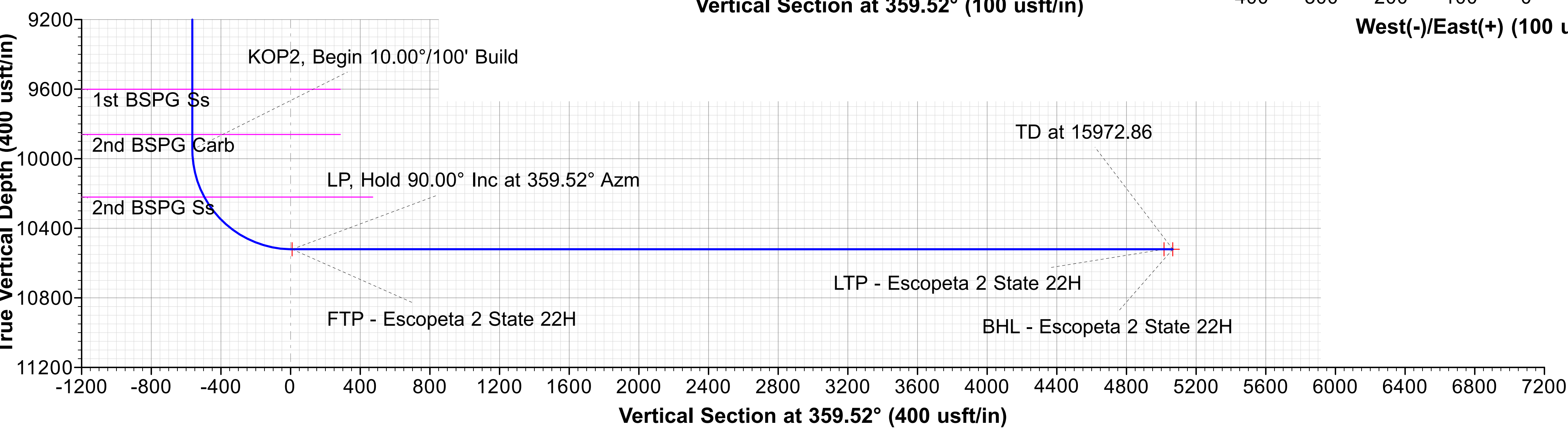
Vertical Section at 359.52° (400 usft/in)
