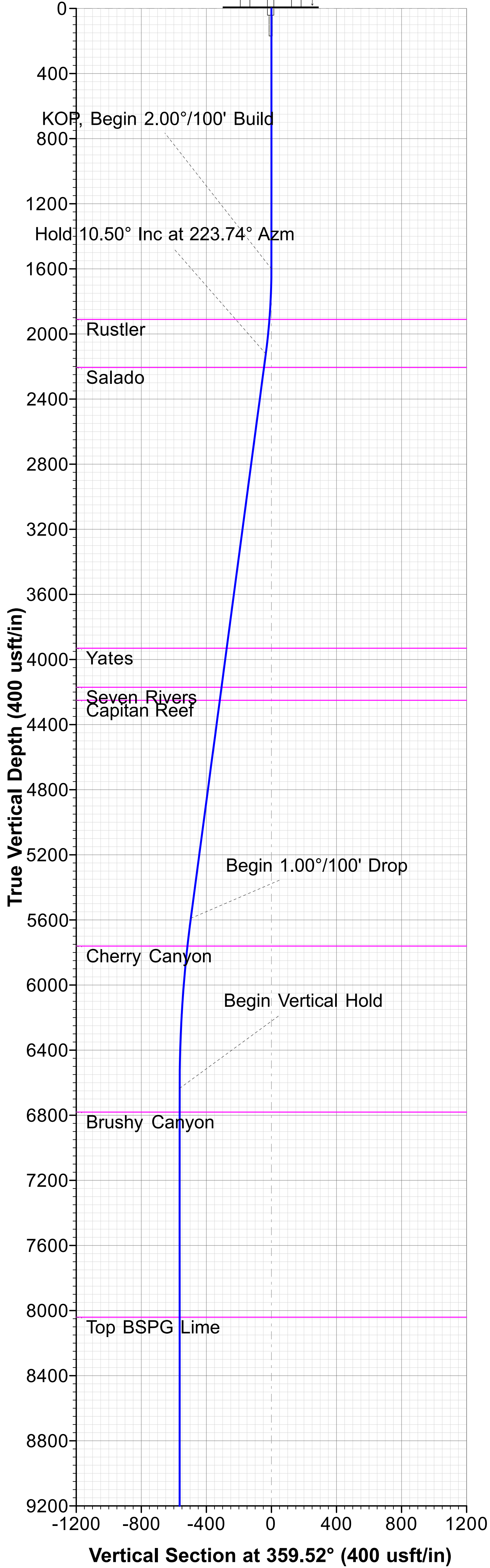
Vertical Section at 359.52° (400 usft/in)
