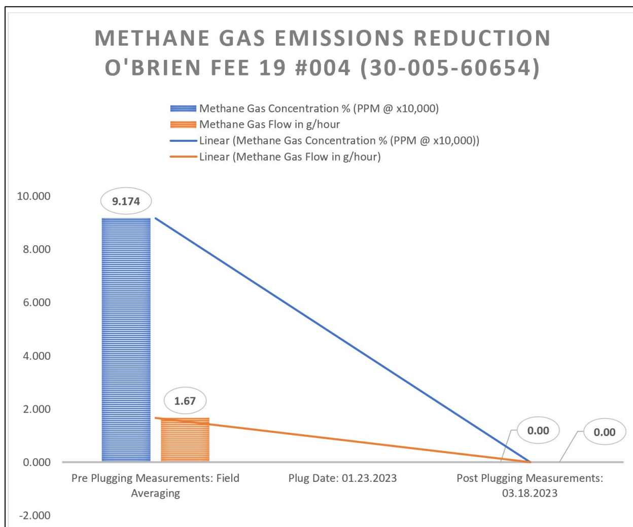
Image 3.1 – O'Brien Fee 19 #004 (30-005-60654) Methane Gas Emissions Reduction Pre Plugging to Post Plugging
