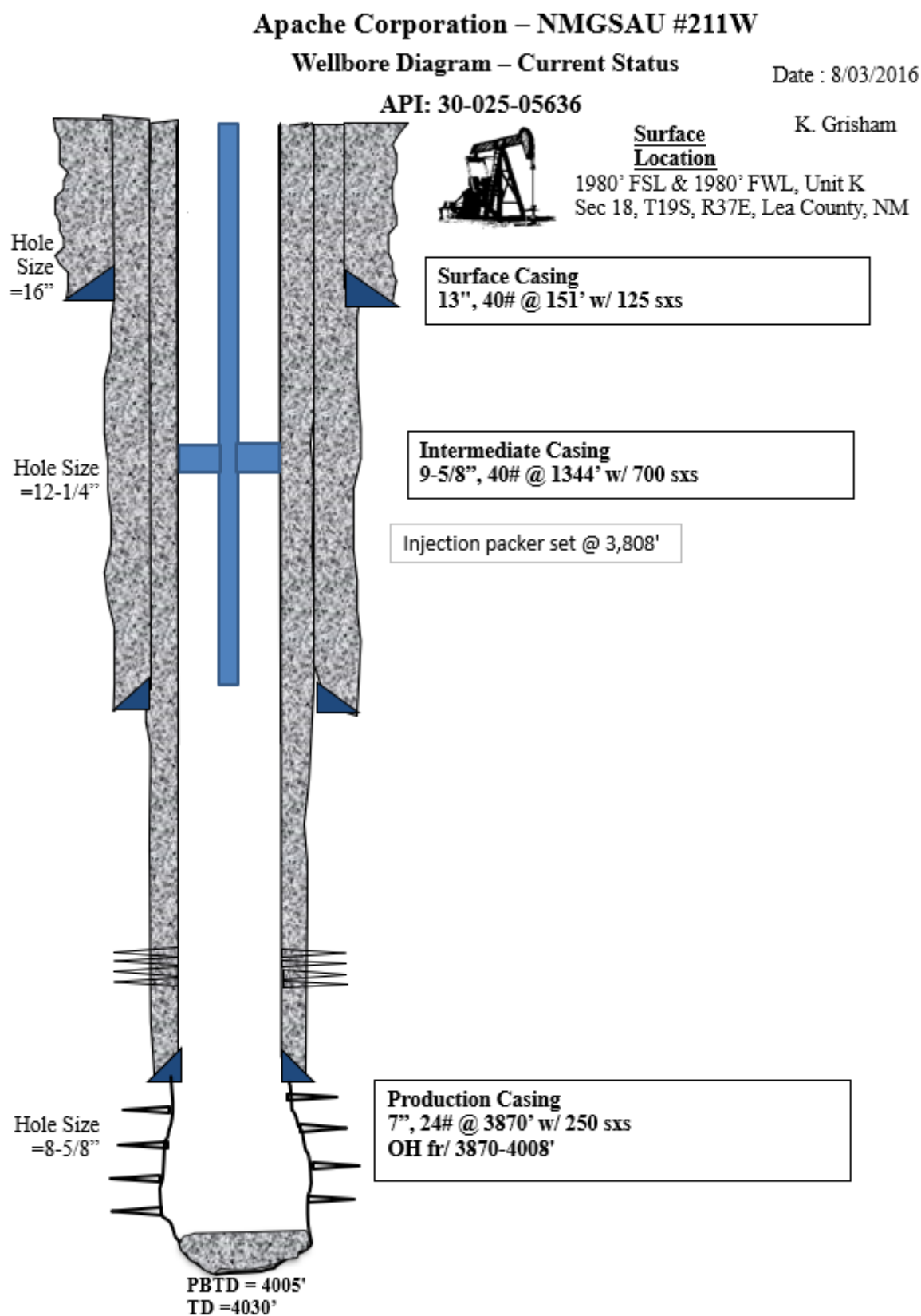
Figure 1 – Current Wellbore Diagram
