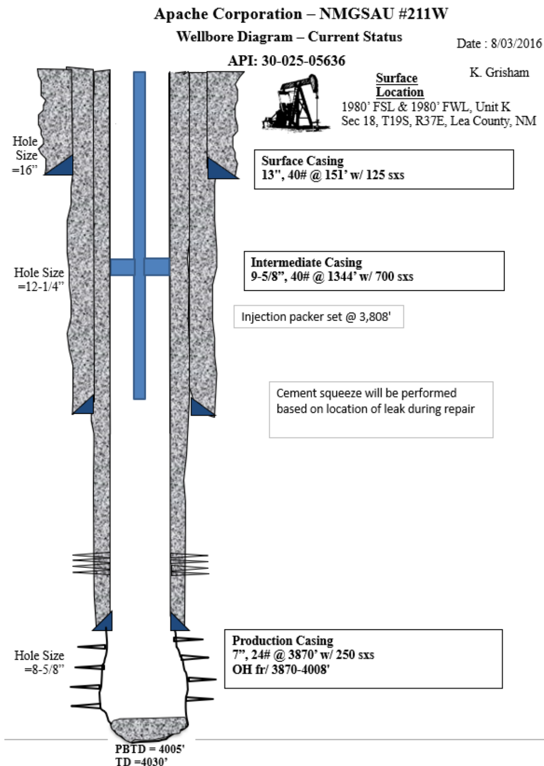
Figure 2 – Proposed Wellbore Diagram
